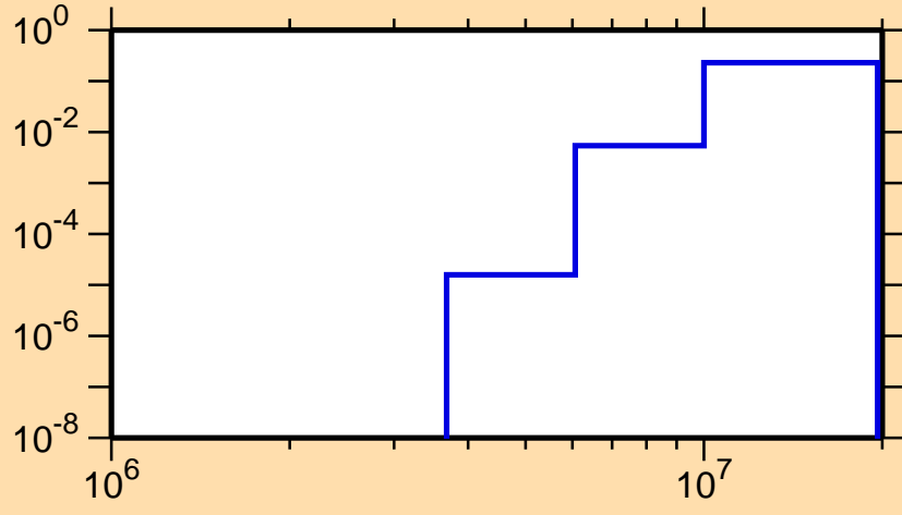
\sigma vs. E for ^{64}\text{Ge}(n,p\alpha)
