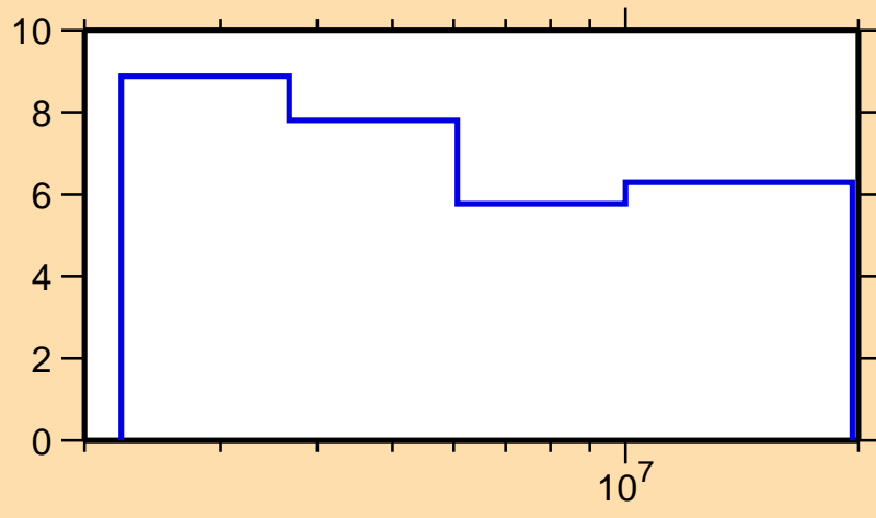
\Delta\sigma/\sigma vs. E for ^{64}\text{Ge}(n,n\text{onel.})
