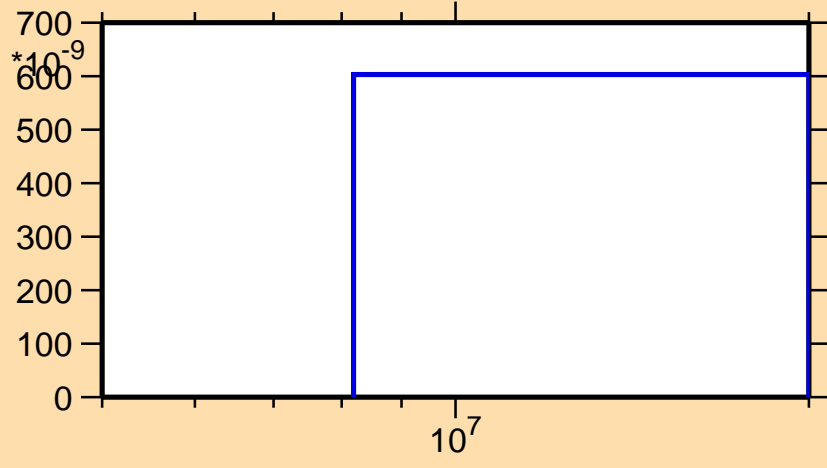
\sigma vs. E for ^{64}\text{Ge}(n,2n)
