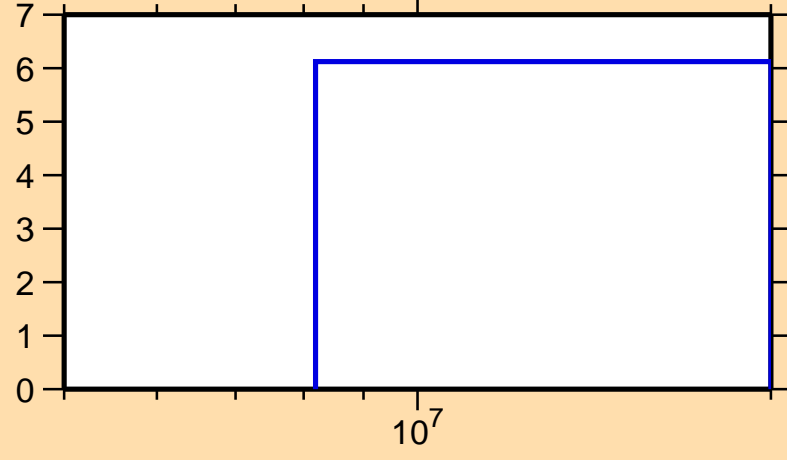
\Delta\sigma/\sigma vs. E for ^{64}\text{Ge}(n,\text{nonel.})
