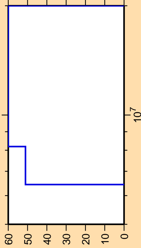
\Delta\sigma/\sigma vs. E for ^{64}\text{Ge}(n,\text{pd})
