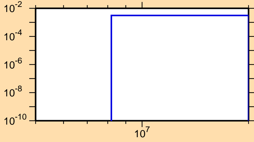
\sigma vs. E for ^{64}\text{Ge}(n,\text{pd})
