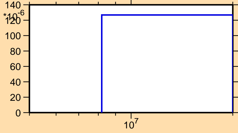
\sigma vs. E for ^{64}\text{Ge}(n,t)
