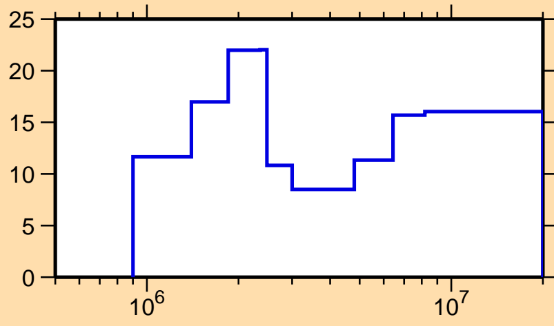
\Delta\sigma/\sigma vs. E for ^{64}\text{Ge}(n,\text{el.})
