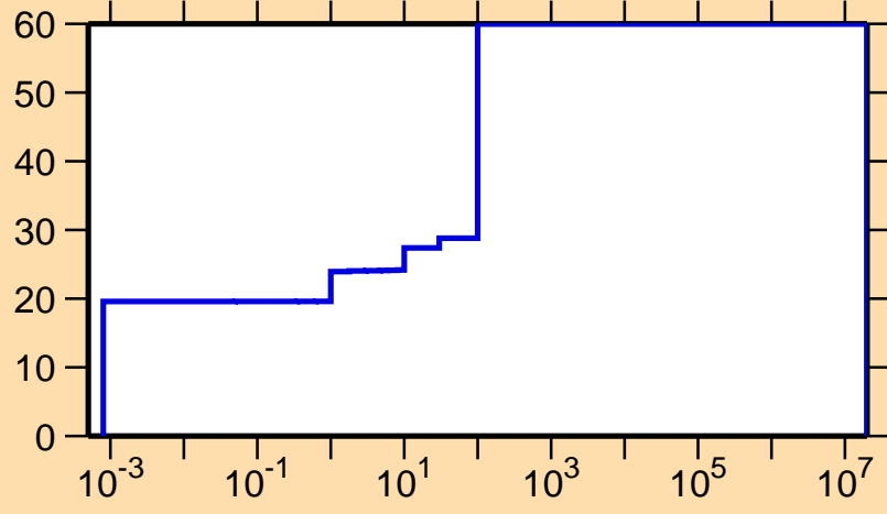
\Delta\sigma/\sigma vs. E for ^{64}\text{Ge}(n,\gamma)
