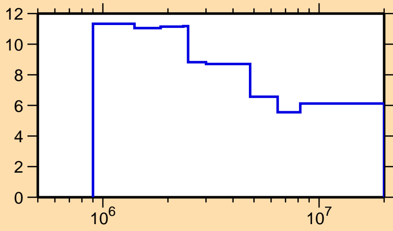
\Delta\sigma/\sigma vs. E for ^{64}\text{Ge}(n,\text{nonel.})
