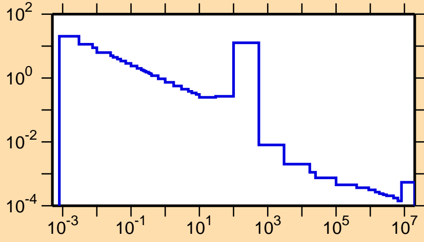
\sigma vs. E for ^{64}\text{Ge}(n,\gamma)
