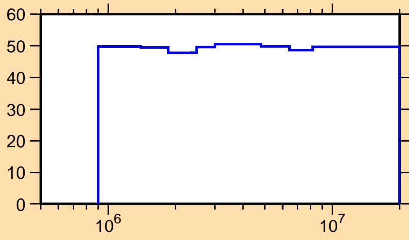
\Delta\sigma/\sigma vs. E for ^{64}\text{Ge}(n,\text{inel.})
