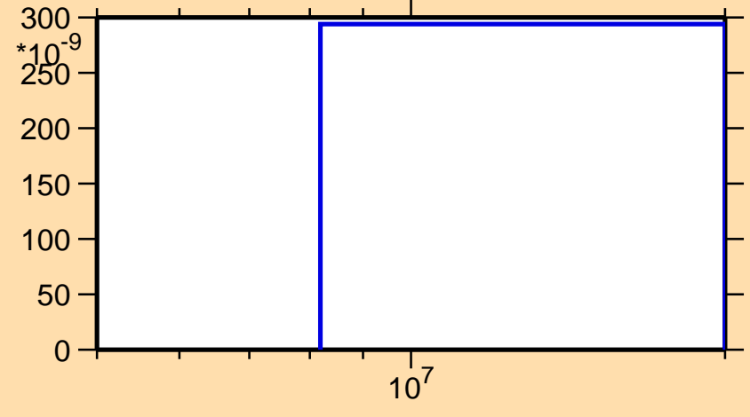
\sigma vs. E for ^{64}\text{Ge}(n,\text{pt})
