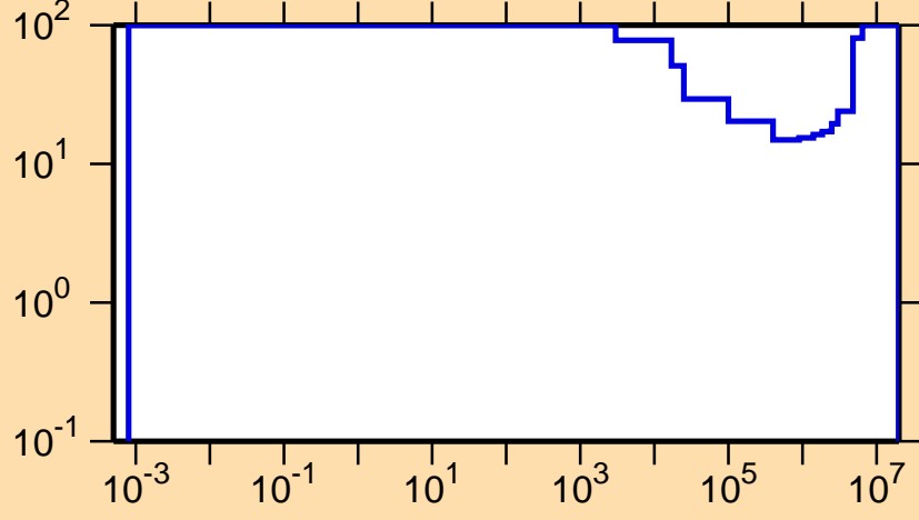
\Delta\sigma/\sigma vs. E for ^{64}\text{Ge}(n,p)
