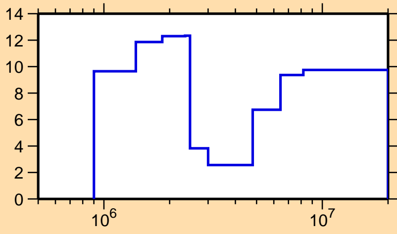
\Delta\sigma/\sigma vs. E for ^{64}\text{Ge}(n,\text{tot.})
