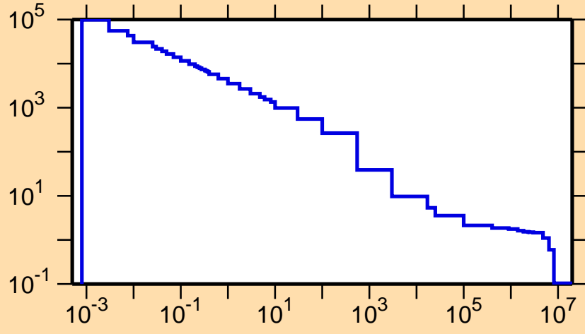
\sigma vs. E for ^{64}\text{Ge}(n,p)
