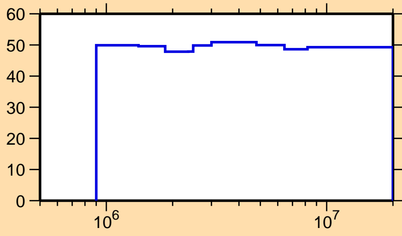
\Delta\sigma/\sigma vs. E for ^{64}\text{Ge}(n,n_1)
