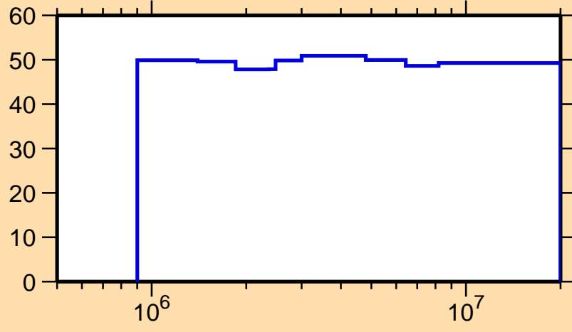
\Delta\sigma/\sigma vs. E for ^{64}\text{Ge}(n,n_1)
