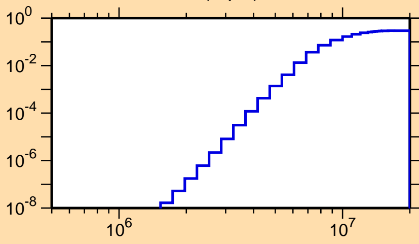
\sigma vs. E for ^{65}\text{Ge}(n,p\alpha)
