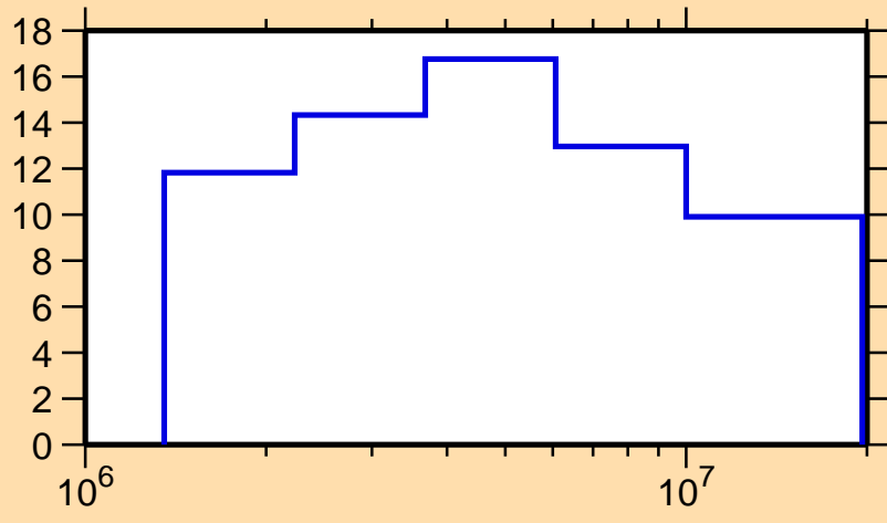
\Delta\sigma/\sigma vs. E for ^{65}\text{Ge}(n,n\text{nonel.})
