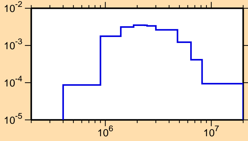
\sigma vs. E for ^{65}\text{Ge}(n,n_3)
