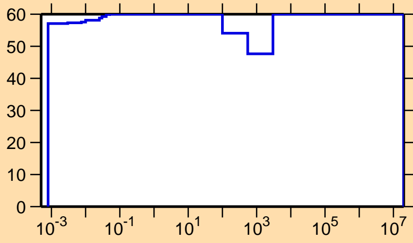
\Delta\sigma/\sigma vs. E for ^{65}\text{Ge}(n,\gamma)
