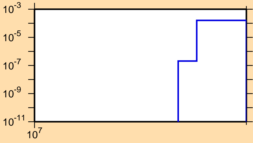
\sigma vs. E for ^{67}\text{Ge}(n,2np)
