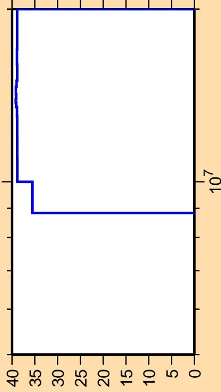
\Delta\sigma/\sigma vs. E for ^{67}\text{Ge}(n,n_1)
