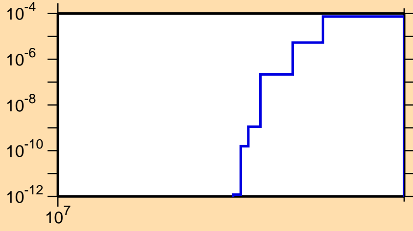
\sigma vs. E for ^{67}\text{Ge}(n,\text{nd})
