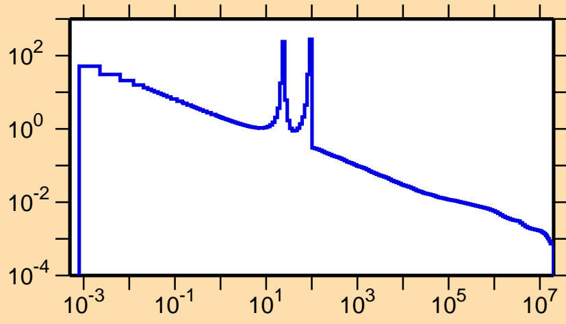
\sigma vs. E for ^{67}\text{Ge}(n,\gamma)
