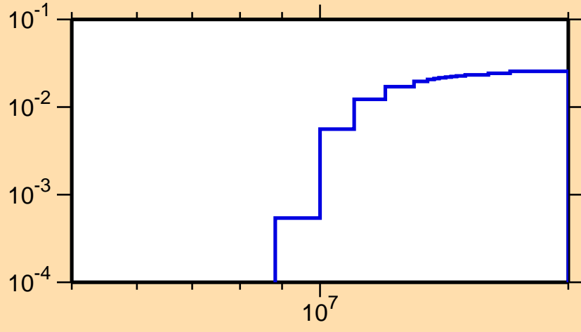
\sigma vs. E for ^{67}\text{Ge}(n,2n)
