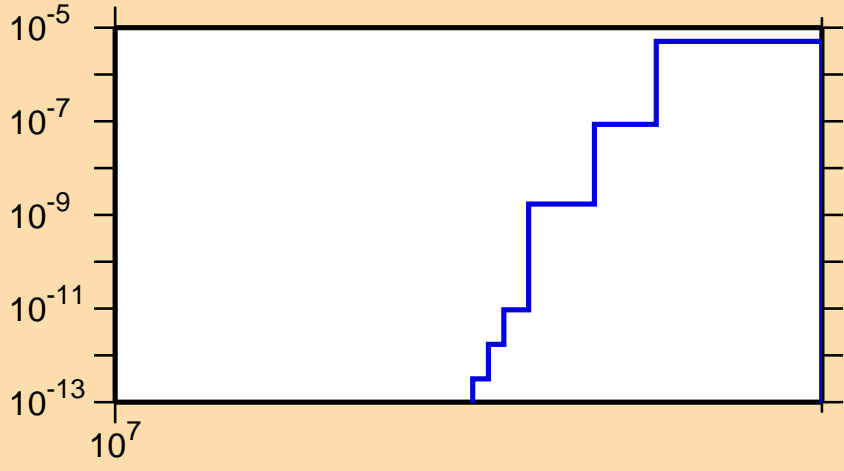
\sigma vs. E for ^{67}\text{Ge} (mt 45)
