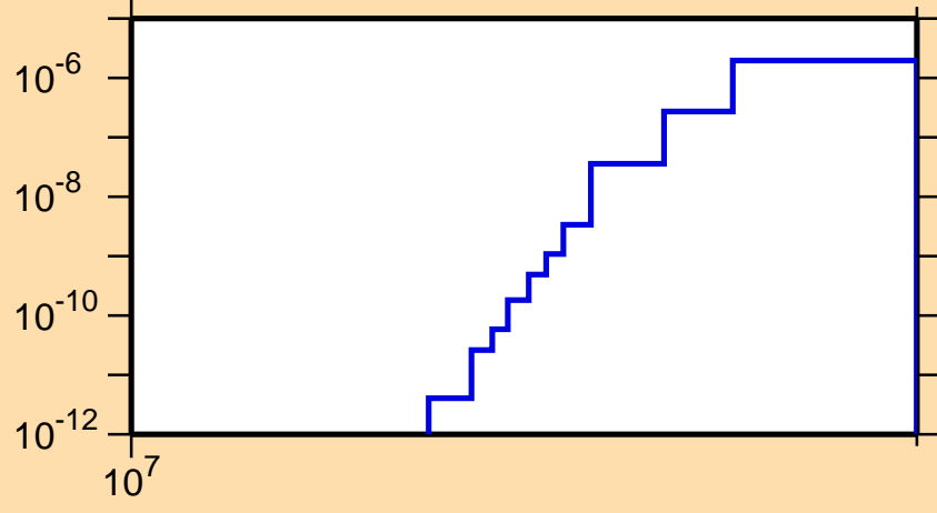
\sigma vs. E for ^{67}\text{Ge}(\text{mt117})
