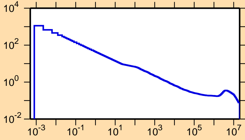
\sigma vs. E for ^{67}\text{Ge}(n,\alpha)
