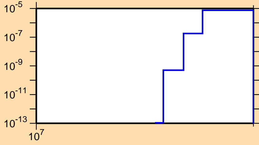
\sigma vs. E for ^{67}\text{Ge}(n,2n\alpha)
