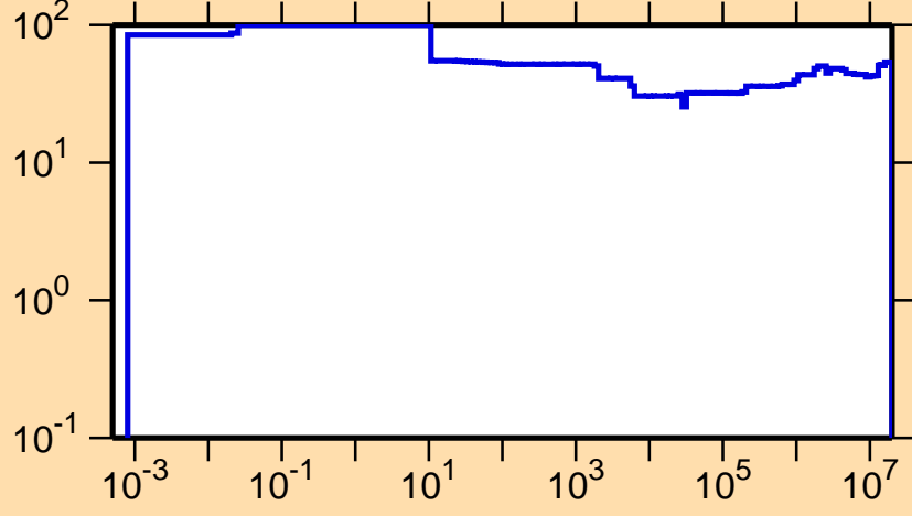
\Delta\sigma/\sigma vs. E for ^{67}\text{Ge}(n,p)
