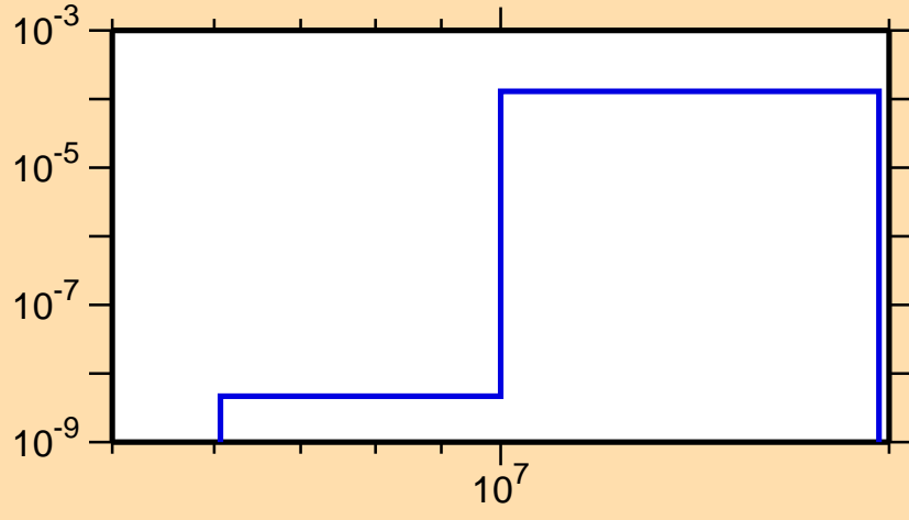
\sigma vs. E for ^{67}\text{Ge}(n,\text{He3})
