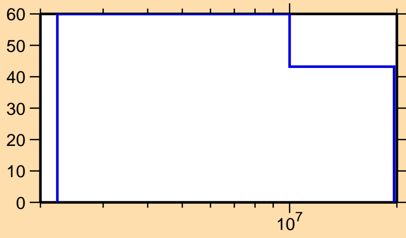
\Delta\sigma/\sigma vs. E for ^{67}\text{Ge}(n,n\text{cont.})
