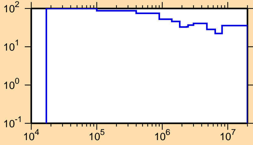
\Delta\sigma/\sigma vs. E for ^{67}\text{Ge}(n,n_1)
