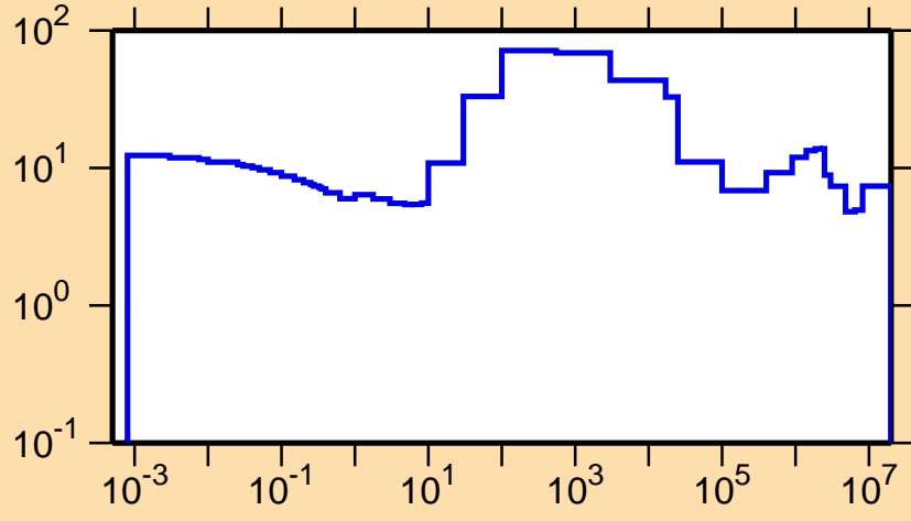
\Delta\sigma/\sigma vs. E for ^{67}\text{Ge}(n,\text{tot.})
