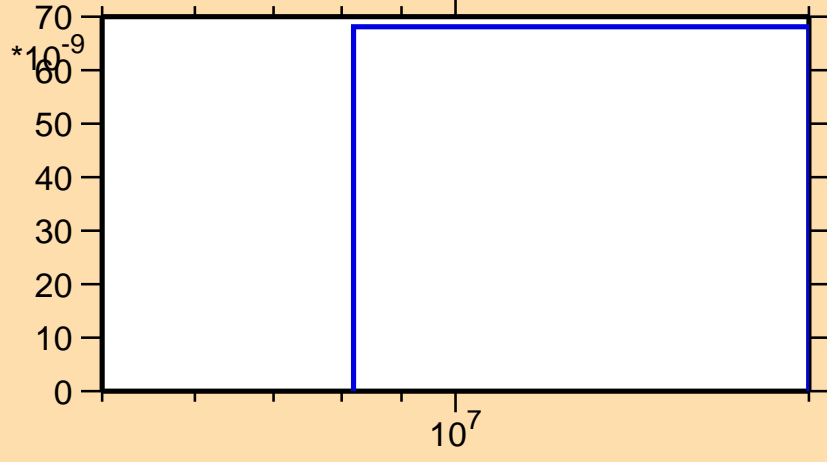
\sigma vs. E for ^{67}\text{Ge}(n,2n\alpha)
