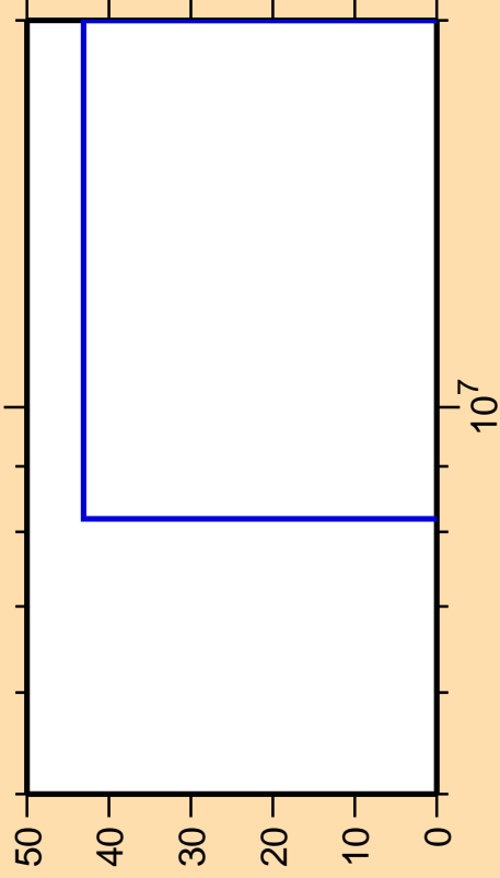
\Delta\sigma/\sigma vs. E for ^{67}\text{Ge}(n,p)
