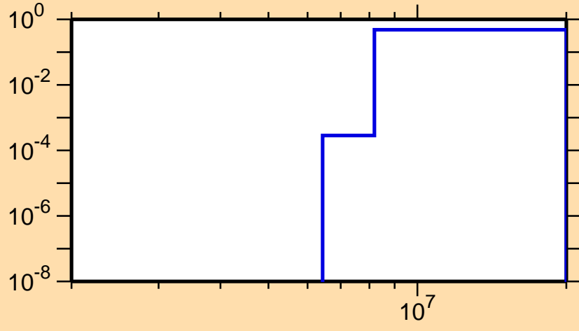
\sigma vs. E for ^{67}\text{Ge}(n,np)
