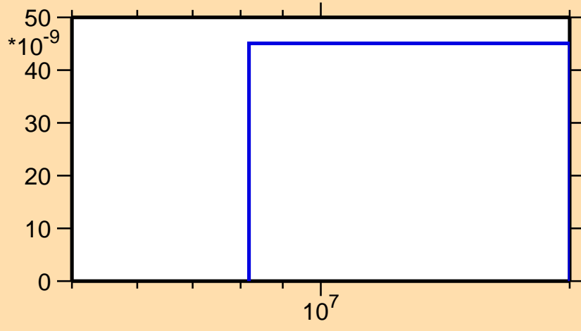
\sigma vs. E for ^{67}\text{Ge} (mt 45)
