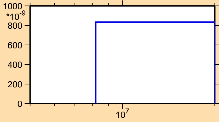
\sigma vs. E for ^{67}\text{Ge}(n,\text{nd})
