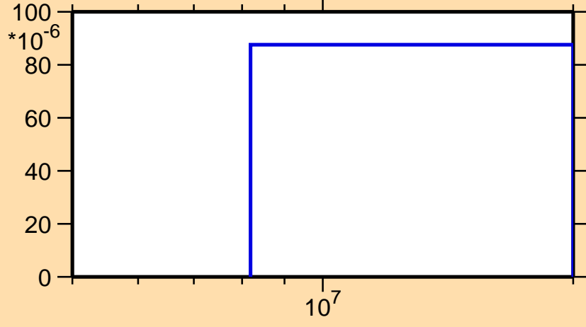
\sigma vs. E for ^{67}\text{Ge}(n,\text{pd})
