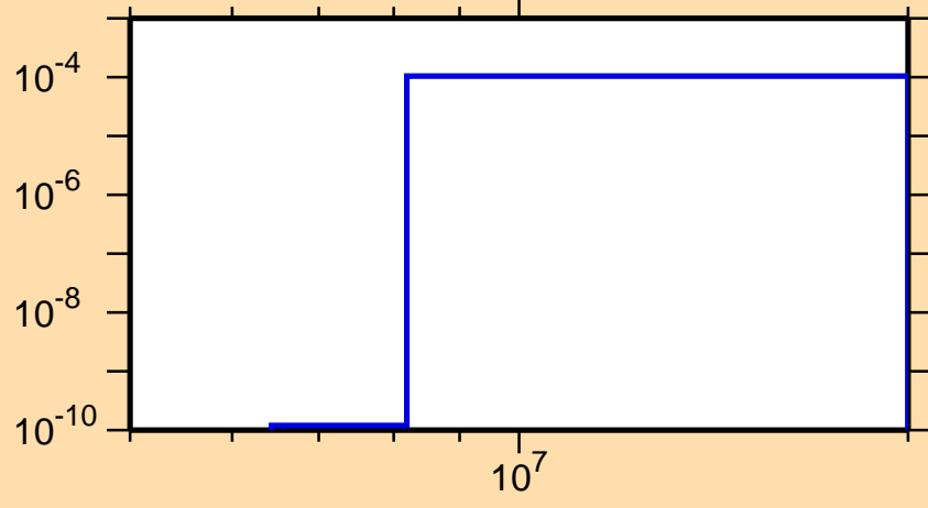
\sigma vs. E for ^{67}\text{Ge}(n,\text{He3})
