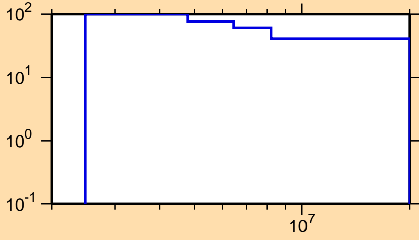
\Delta\sigma/\sigma vs. E for ^{67}\text{Ge}(n,n\text{cont.})
