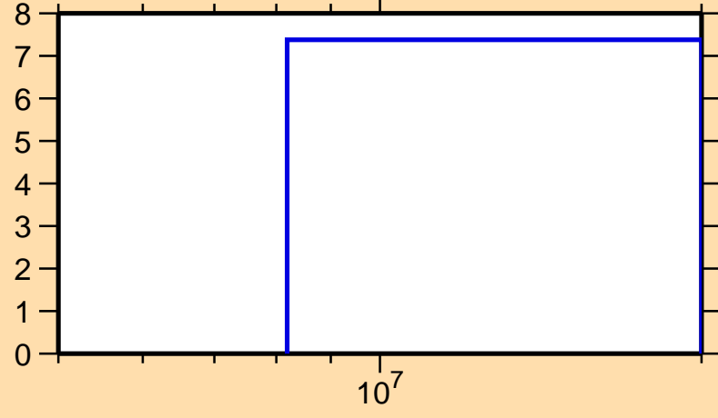
\Delta\sigma/\sigma vs. E for ^{67}\text{Ge}(n,\text{tot.})
