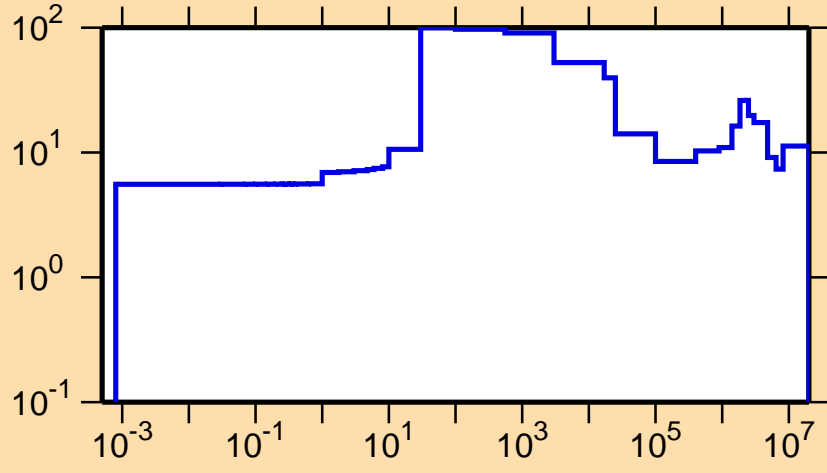
\Delta\sigma/\sigma vs. E for ^{67}\text{Ge}(n,\text{el.})
