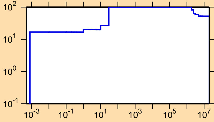
\Delta\sigma/\sigma vs. E for ^{67}\text{Ge}(n,\gamma)
