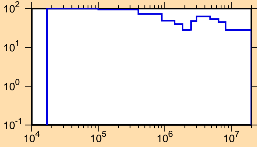
\Delta\sigma/\sigma vs. E for ^{67}\text{Ge}(n,\text{inel.})
