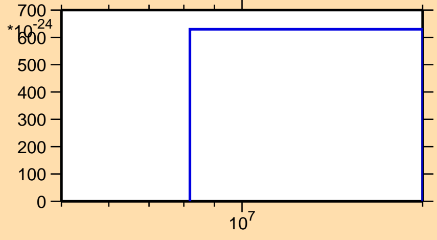
\sigma vs. E for ^{67}\text{Ge}(n,nt)
