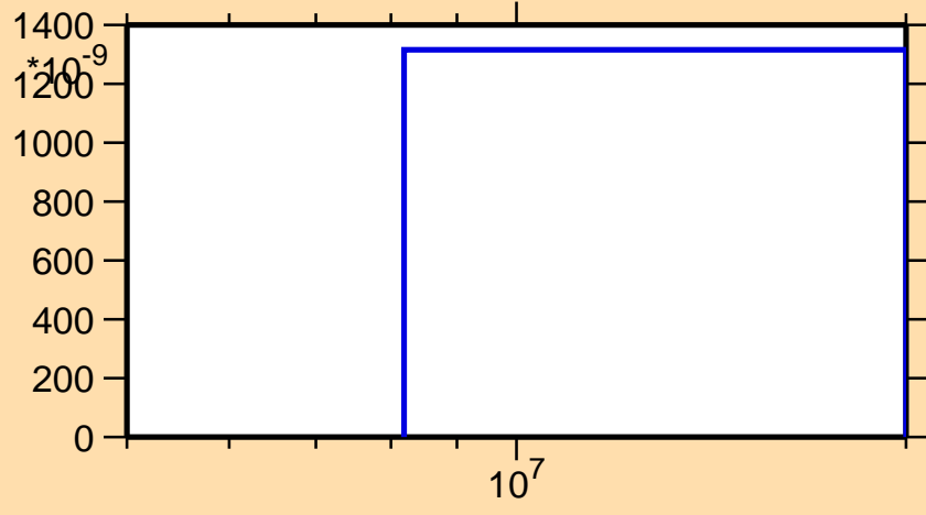
\sigma vs. E for ^{67}\text{Ge}(n,2np)
