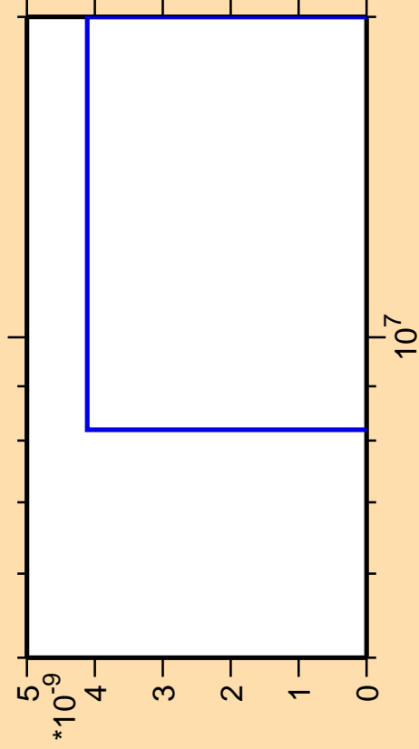
\Delta\sigma/\sigma vs. E for ^{67}\text{Ge}(n,nt)
