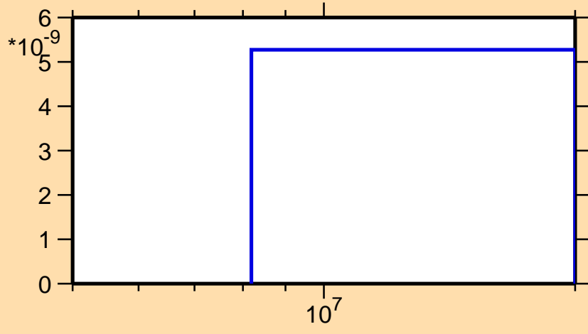
\sigma vs. E for ^{67}\text{Ge} (mt 34)
