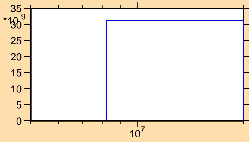
\sigma vs. E for ^{67}\text{Ge}(\text{mt117})
