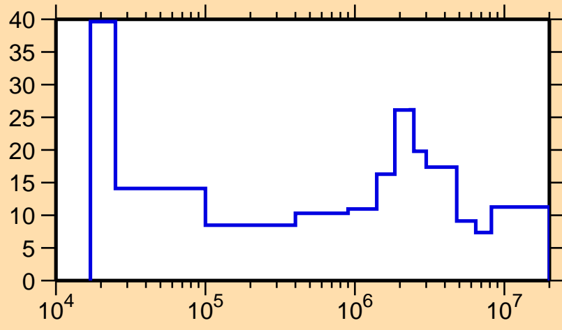
\Delta\sigma/\sigma vs. E for ^{67}\text{Ge}(n,\text{el.})
