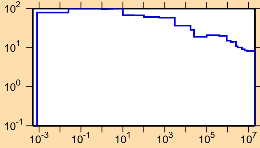
\Delta\sigma/\sigma vs. E for ^{67}\text{Ge}(n,\text{nonel.})
