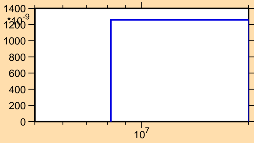
\sigma vs. E for ^{67}\text{Ge}(n,\text{pt})
