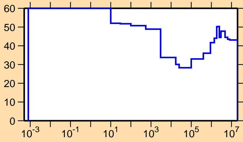
\Delta\sigma/\sigma vs. E for ^{67}\text{Ge}(n,p)
