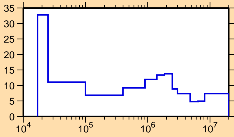
\Delta\sigma/\sigma vs. E for ^{67}\text{Ge}(n,\text{tot.})
