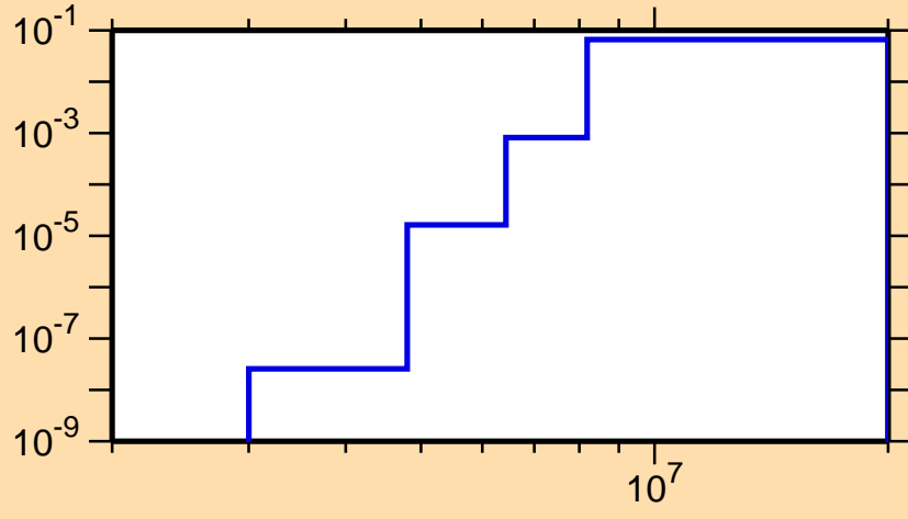
\sigma vs. E for ^{67}\text{Ge}(n,p\alpha)
