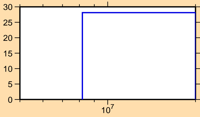
\Delta\sigma/\sigma vs. E for ^{67}\text{Ge}(n,\text{inel.})
