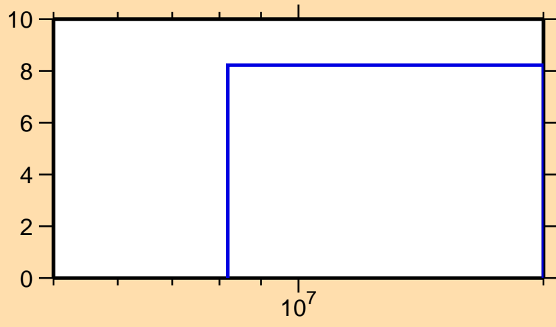
\Delta\sigma/\sigma vs. E for ^{67}\text{Ge}(n,\text{nonel.})
