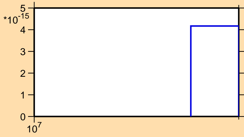
\sigma vs. E for ^{68}\text{Ge}(n,nt)
