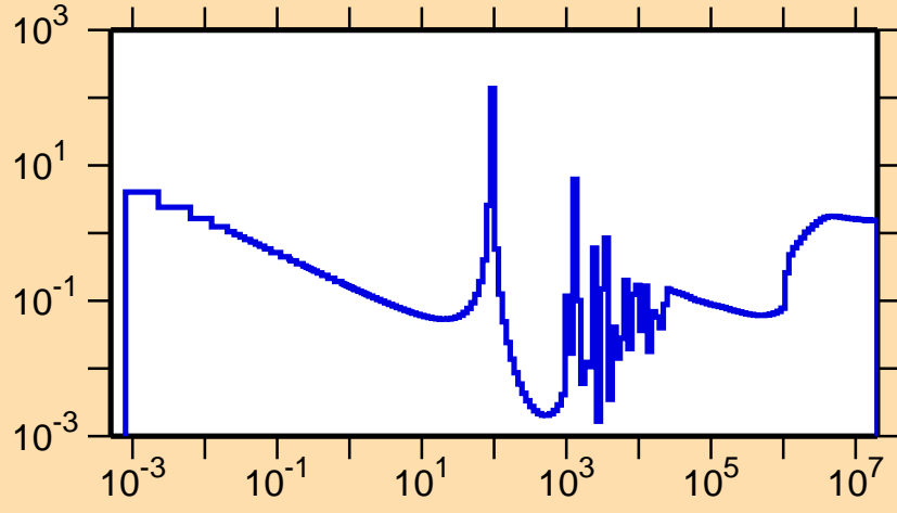
\sigma vs. E for ^{68}\text{Ge}(n,\text{nonel.})
