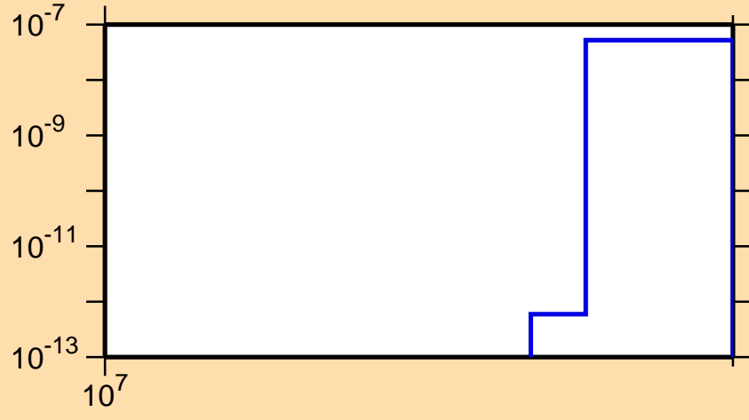
\sigma vs. E for ^{68}\text{Ge}(n,\text{nd})
