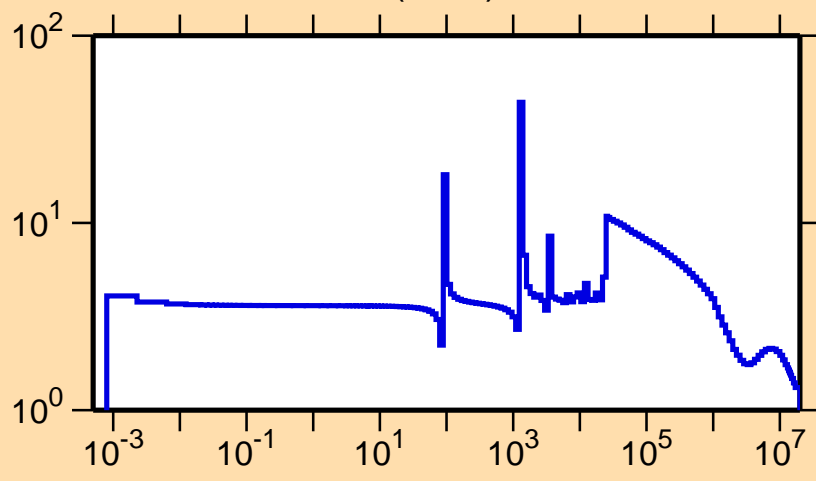
\sigma vs. E for ^{68}\text{Ge}(n,\text{el.})
