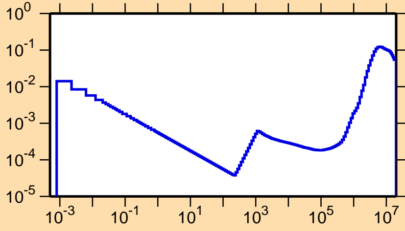
\sigma vs. E for ^{68}\text{Ge}(n,\alpha)
