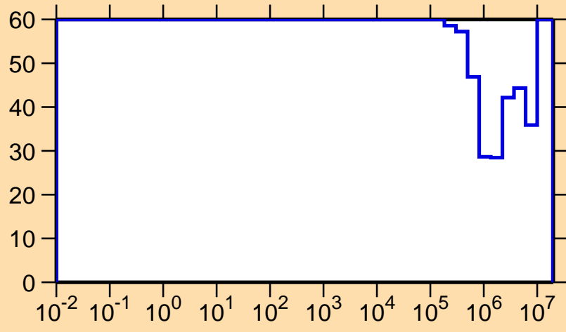
\Delta\sigma/\sigma vs. E for ^{68}\text{Ge}(n,p)
