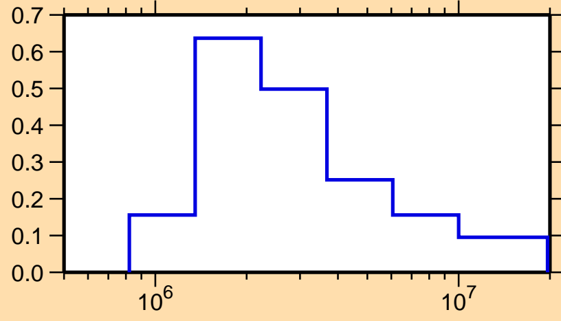
\sigma vs. E for ^{68}\text{Ge}(n,n_1)
