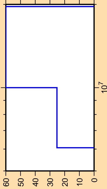
\Delta\sigma/\sigma vs. E for ^{68}\text{Ge}(n,\text{He}3)
