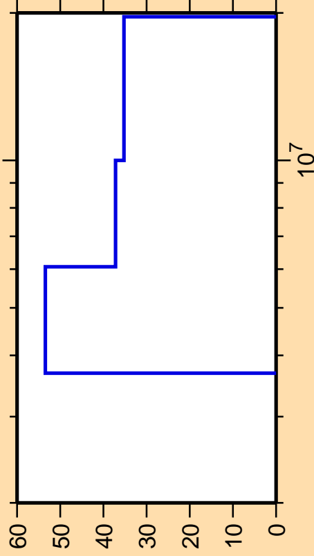
\Delta\sigma/\sigma vs. E for ^{68}\text{Ge}(n,n\text{cont.})
