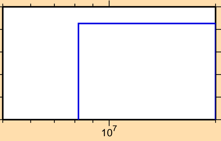
\sigma vs. E for ^{68}\text{Ge}(n,\text{nd})
