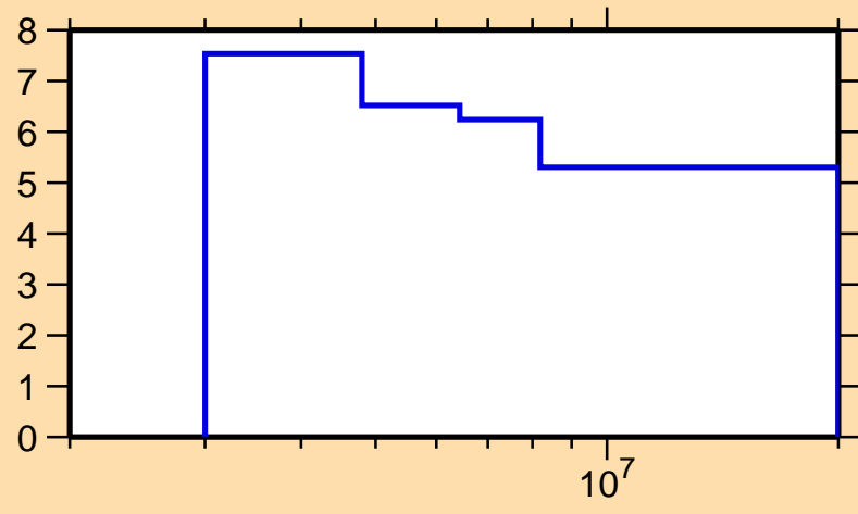
\Delta\sigma/\sigma vs. E for ^{68}\text{Ge}(n,n\text{onel.})
