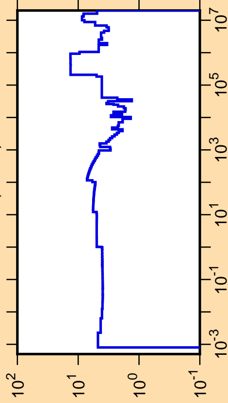
\Delta\sigma/\sigma vs. E for ^{70}\text{Ge}(n,\text{tot.})
