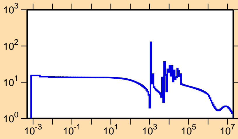
\sigma vs. E for ^{70}\text{Ge}(n,\text{el.})
