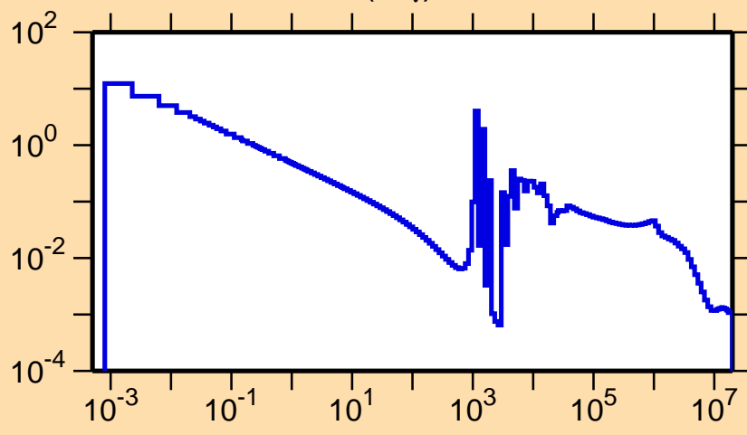
\sigma vs. E for ^{70}\text{Ge}(n,\gamma)
