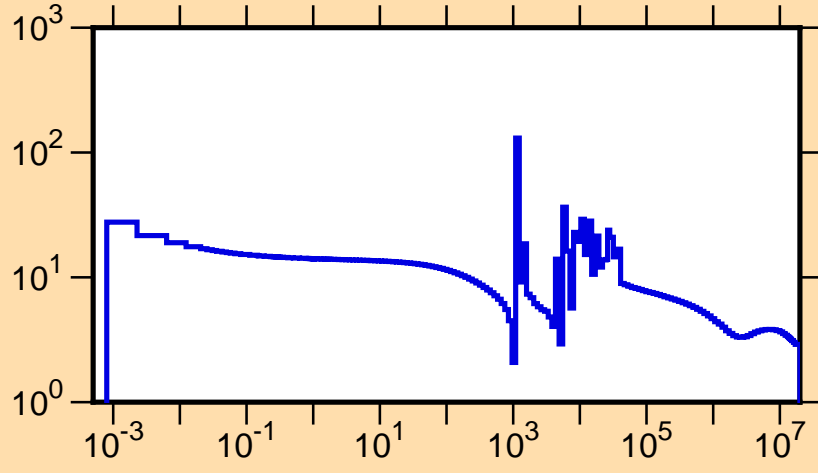
\sigma vs. E for ^{70}\text{Ge}(n,\text{tot.})
