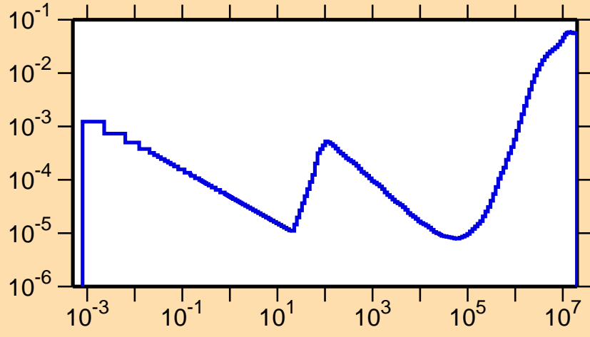
\sigma vs. E for ^{71}\text{Ge}(n,p)
