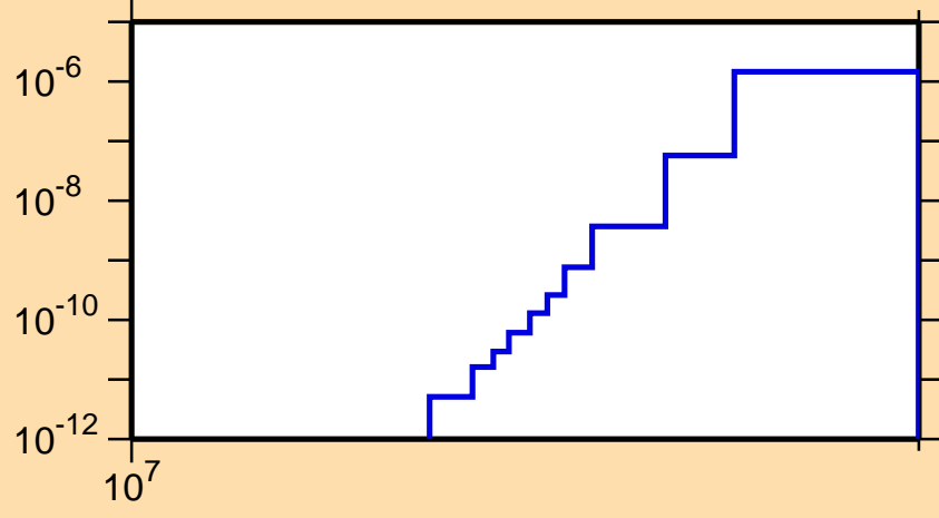
\sigma vs. E for ^{71}\text{Ge}(n,\text{He}3)
