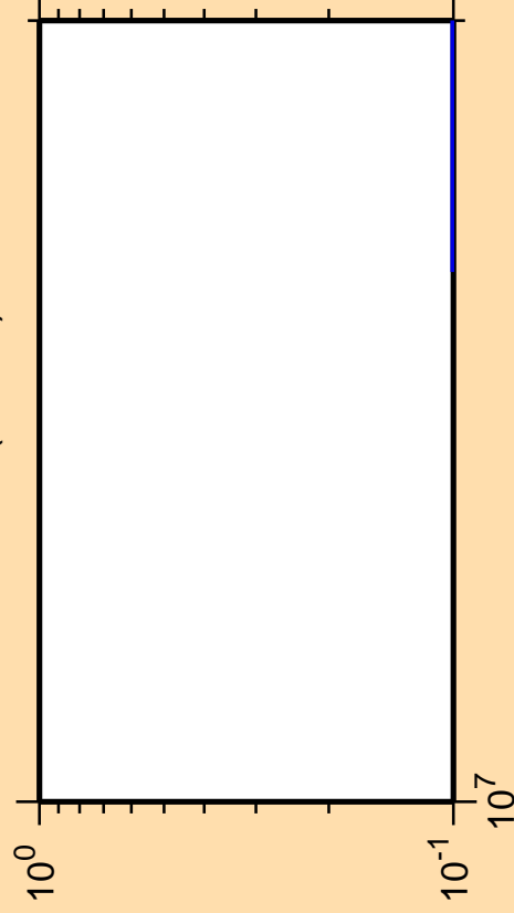
\Delta\sigma/\sigma vs. E for ^{71}\text{Ge} (mt 45)
