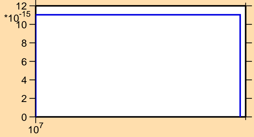
\sigma vs. E for ^{71}\text{Ge} (mt117)
