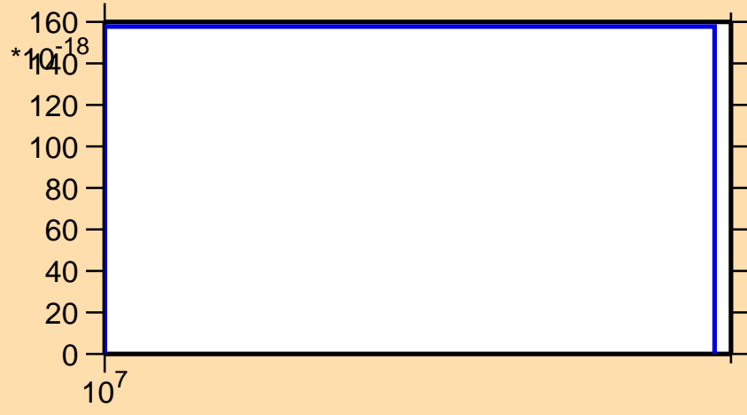
\sigma vs. E for ^{71}\text{Ge} (mt 45)
