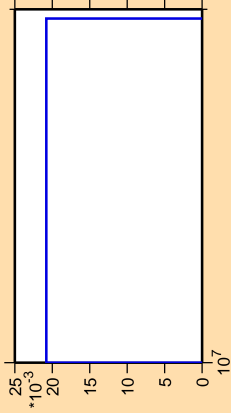
\Delta\sigma/\sigma vs. E for ^{71}\text{Ge} (mt117)
