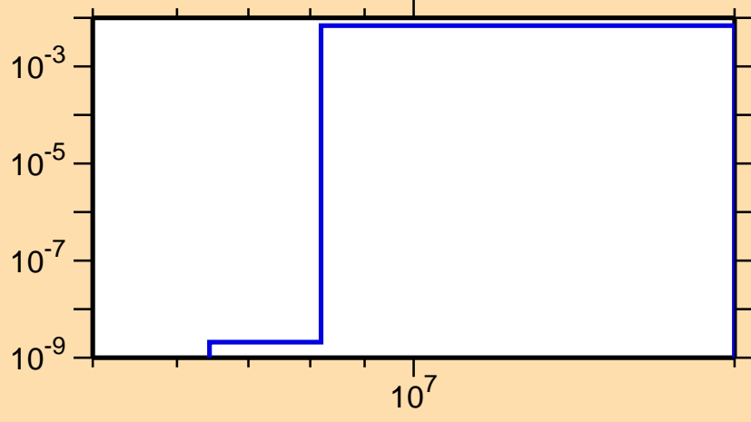
\sigma vs. E for ^{71}\text{Ge}(n,n\alpha)
