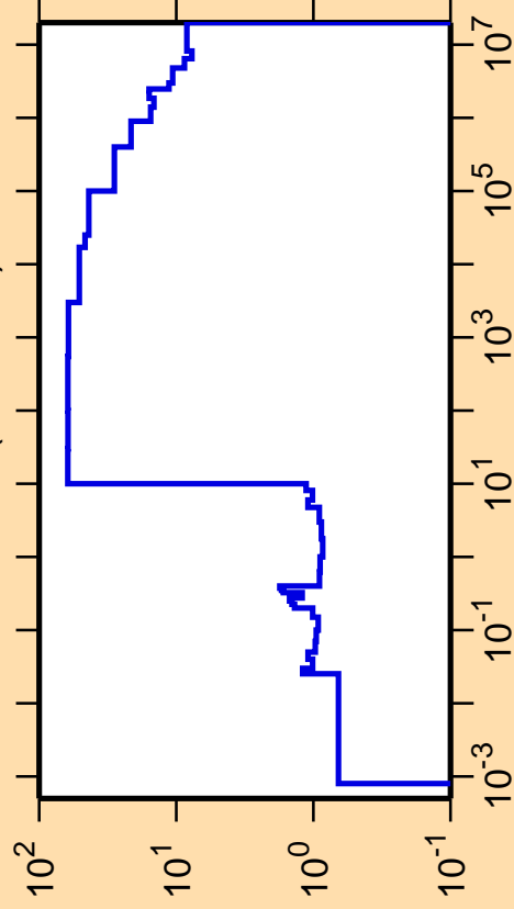
\Delta\sigma/\sigma vs. E for ^{71}\text{Ge}(n,\text{nonel.})
