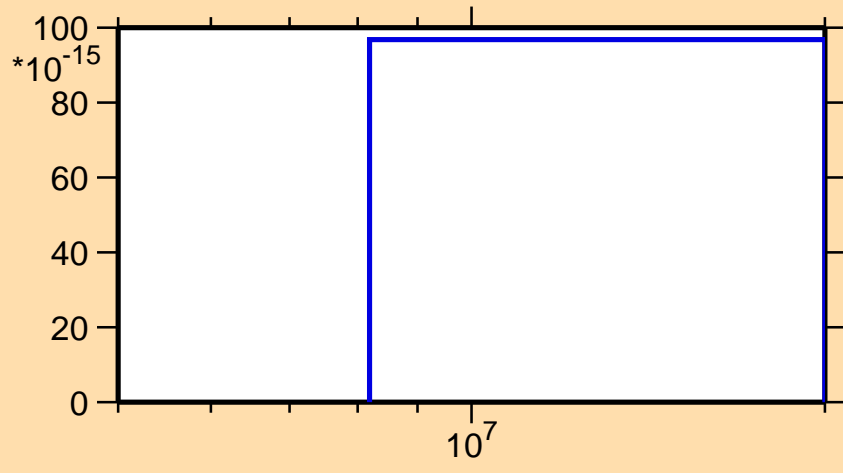
\sigma vs. E for ^{71}\text{Ge} (mt 34)
