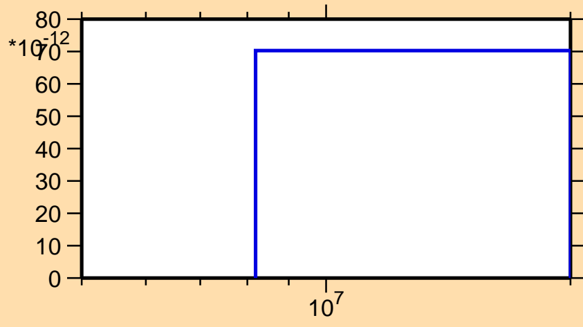
\sigma vs. E for ^{71}\text{Ge}(n,\text{pt})
