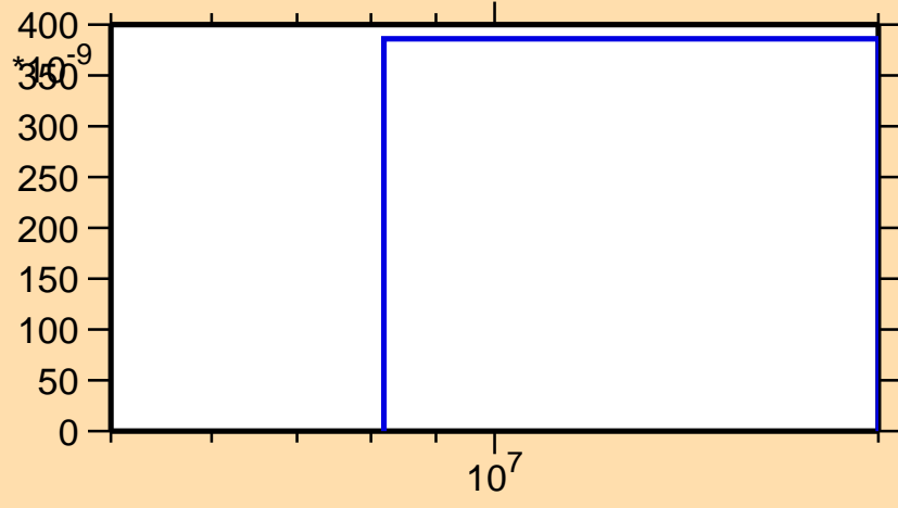
\sigma vs. E for ^{71}\text{Ge}(n,\text{nd})
