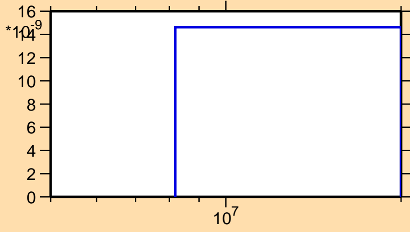
\sigma vs. E for ^{71}\text{Ge}(n,\text{He3})
