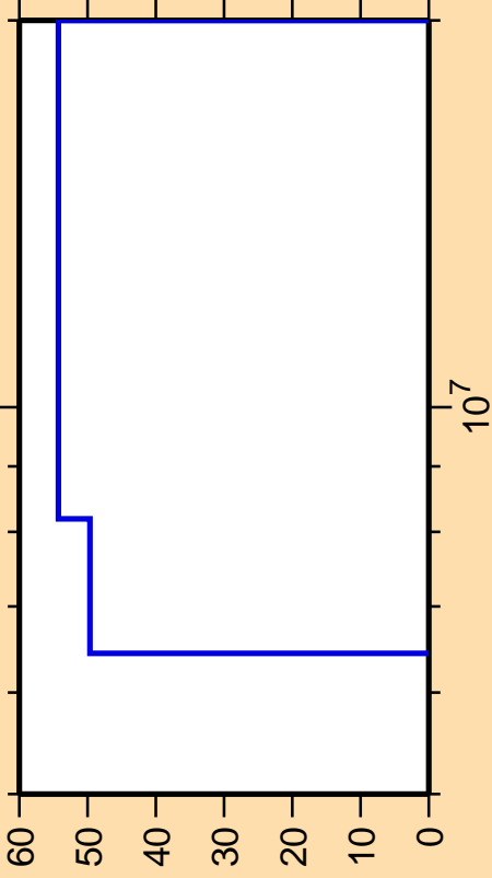
\Delta\sigma/\sigma vs. E for ^{71}\text{Ge}(n,\alpha)
