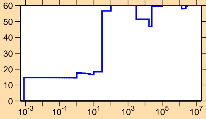
\Delta\sigma/\sigma vs. E for ^{71}\text{Ge}(n,\gamma)
