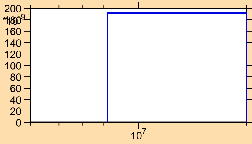
\sigma vs. E for ^{71}\text{Ge}(n,3n)
