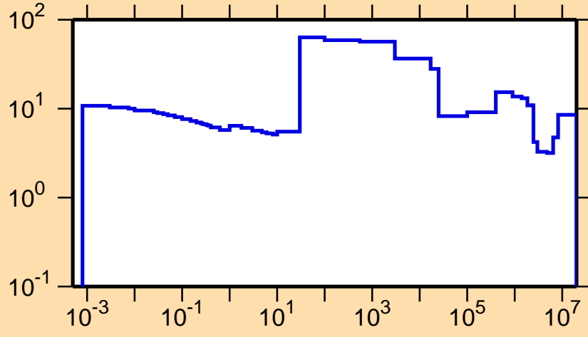
\Delta\sigma/\sigma vs. E for ^{71}\text{Ge}(n,\text{tot.})
