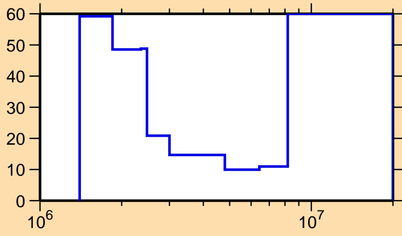
\Delta\sigma/\sigma vs. E for ^{71}\text{Ge}(n,ncont.)
