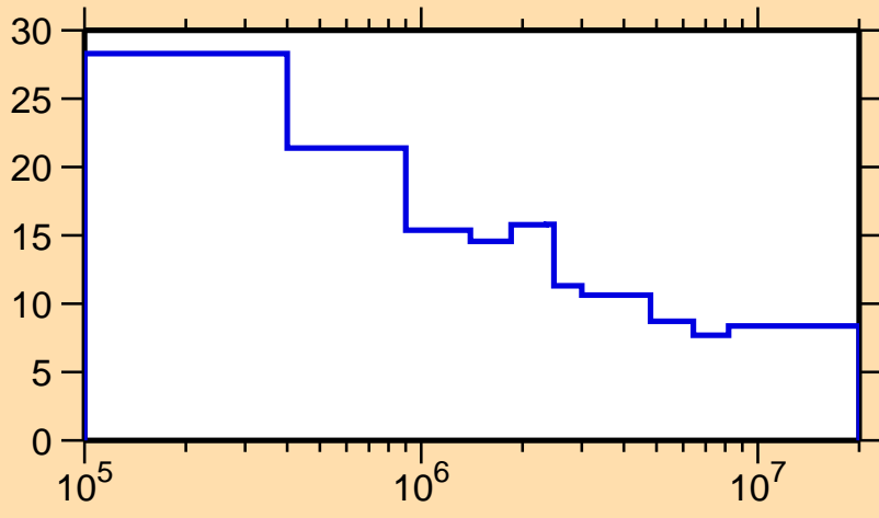
\Delta\sigma/\sigma vs. E for ^{71}\text{Ge}(n,\text{nonel.})
