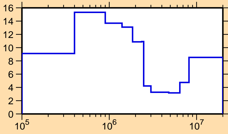
\Delta\sigma/\sigma vs. E for ^{71}\text{Ge}(n,\text{tot.})
