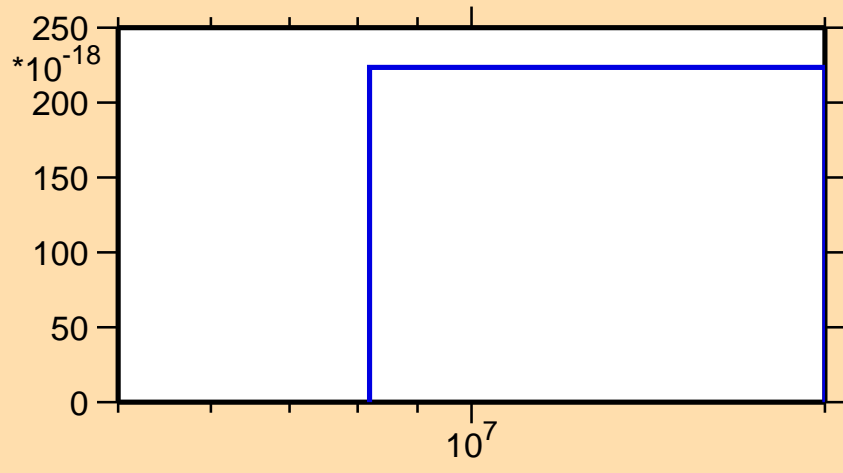
\sigma vs. E for ^{71}\text{Ge} (mt 45)
