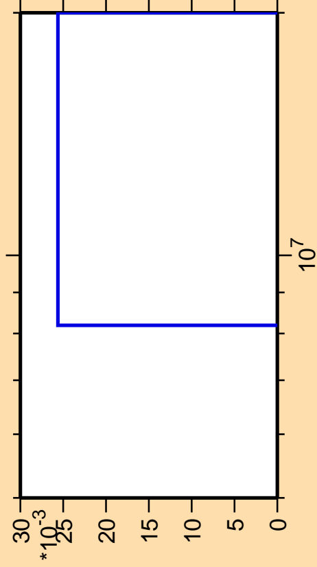
\Delta\sigma/\sigma vs. E for ^{71}\text{Ge}(\text{mt117})
