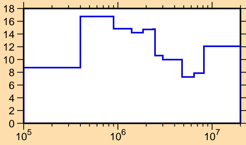
\Delta\sigma/\sigma vs. E for ^{71}\text{Ge}(n,\text{el.})
