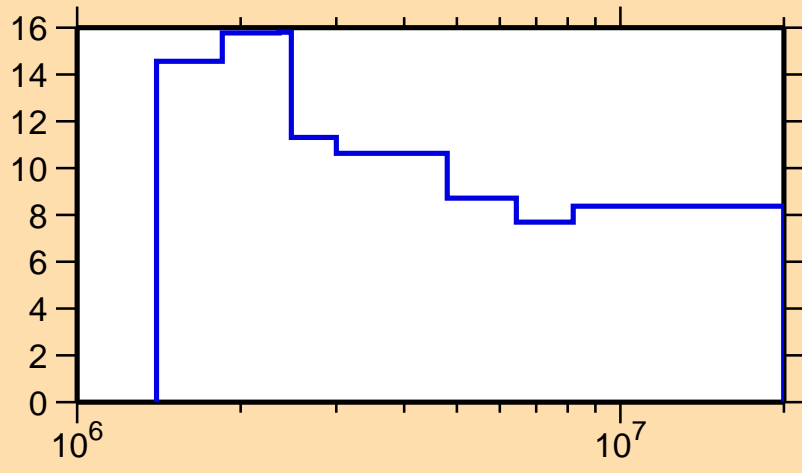
\Delta\sigma/\sigma vs. E for ^{71}\text{Ge}(n,n\text{onel.})
