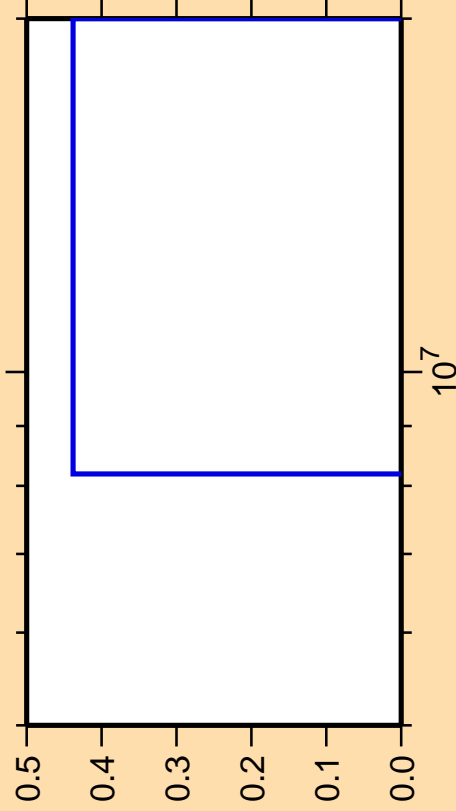
\Delta\sigma/\sigma vs. E for ^{71}\text{Ge} (mt 34)
