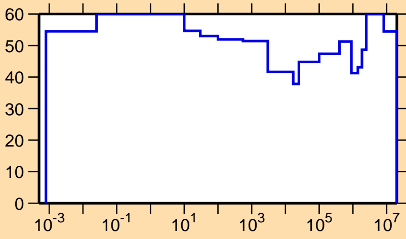
\Delta\sigma/\sigma vs. E for ^{71}\text{Ge}(n,p)
