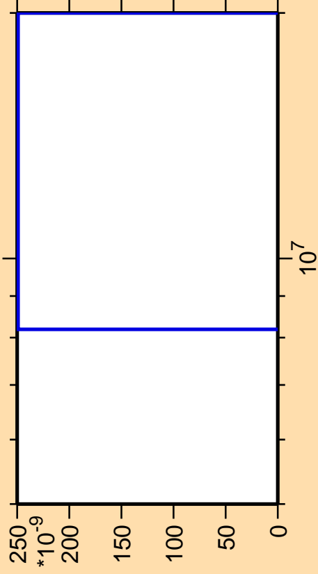
\Delta\sigma/\sigma vs. E for ^{71}\text{Ge} (mt 45)
