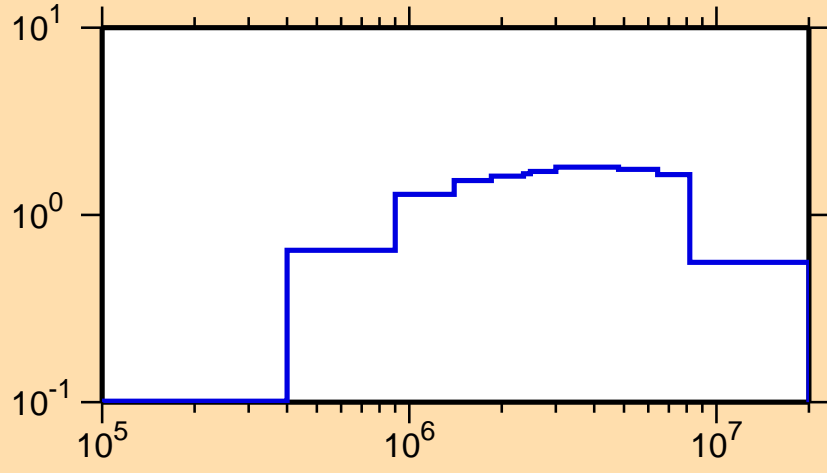
\sigma vs. E for ^{71}\text{Ge}(n,\text{inel.})
