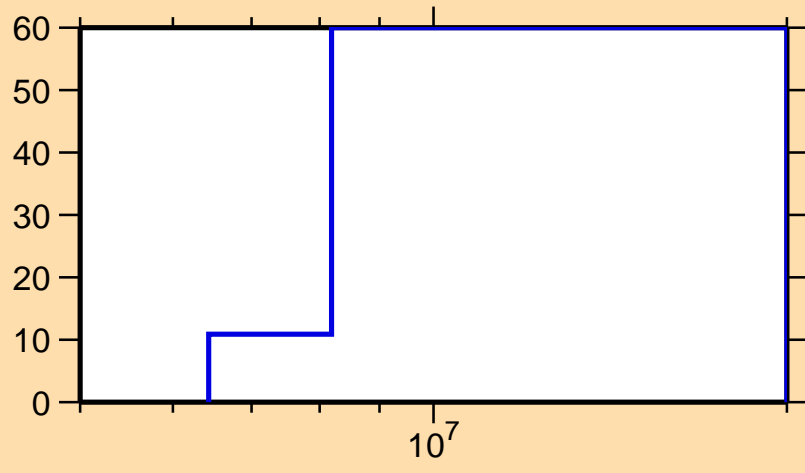
\Delta\sigma/\sigma vs. E for ^{71}\text{Ge}(n,\text{inel.})
