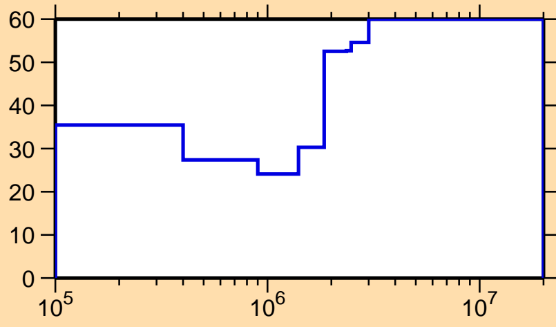
\Delta\sigma/\sigma vs. E for ^{71}\text{Ge}(n,n_1)
