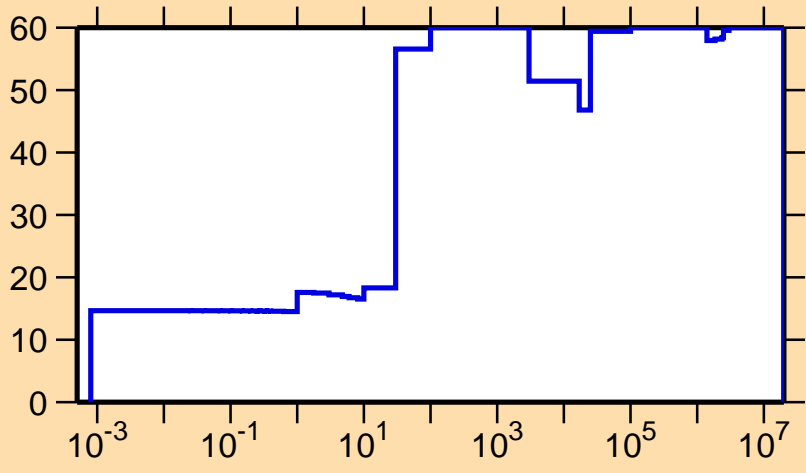
\Delta\sigma/\sigma vs. E for ^{71}\text{Ge}(n,\gamma)
