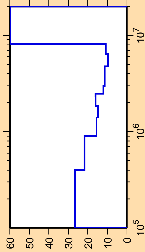
\Delta\sigma/\sigma vs. E for ^{71}\text{Ge}(n,\text{inel.})
