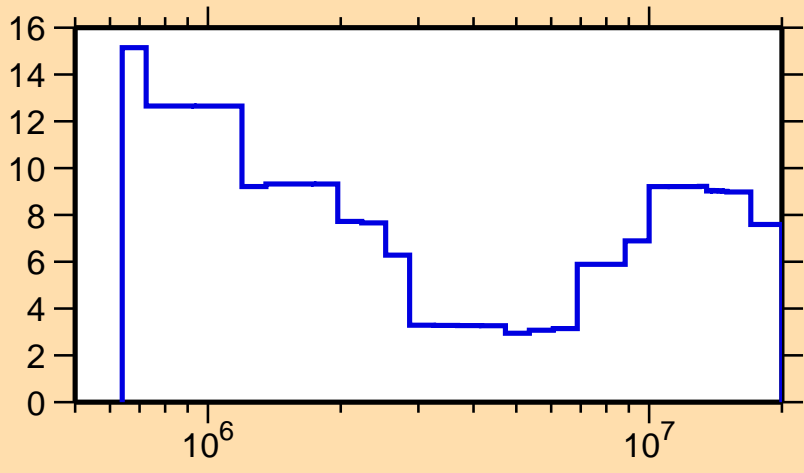
\Delta\sigma/\sigma vs. E for ^{72}\text{Ge}(n,\text{tot.})
