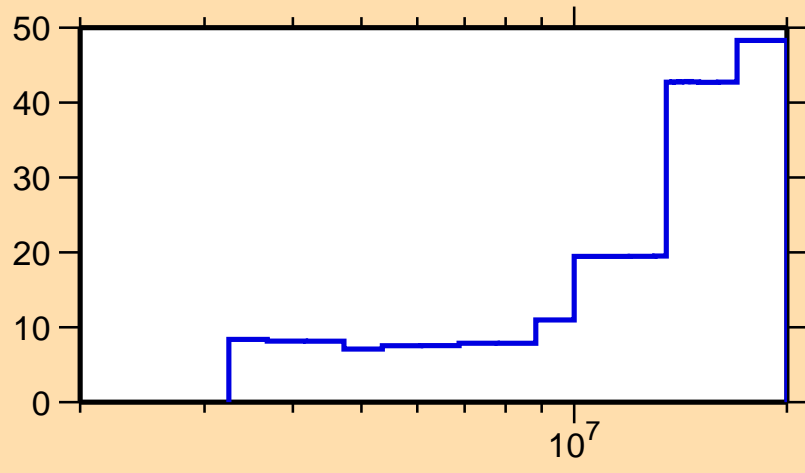
\Delta\sigma/\sigma vs. E for ^{72}\text{Ge}(n,n\text{cont.})
