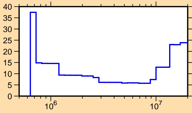
\Delta\sigma/\sigma vs. E for ^{72}\text{Ge}(n,\text{inel.})
