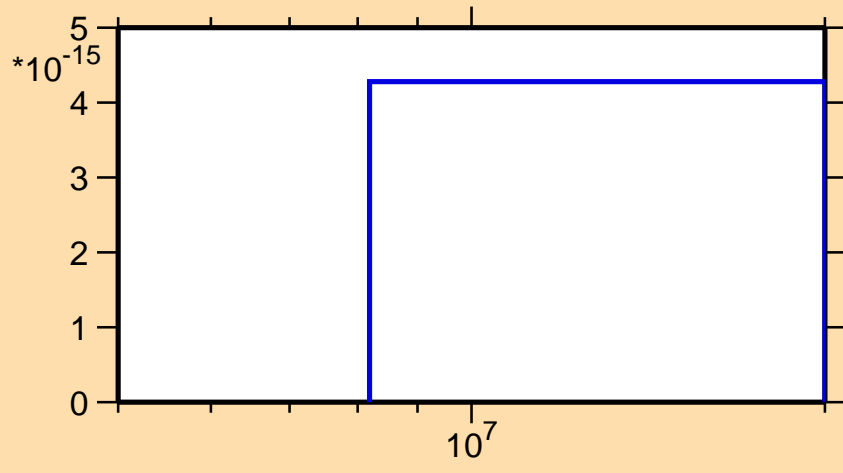
\sigma vs. E for ^{72}\text{Ge}(\text{mt117})
