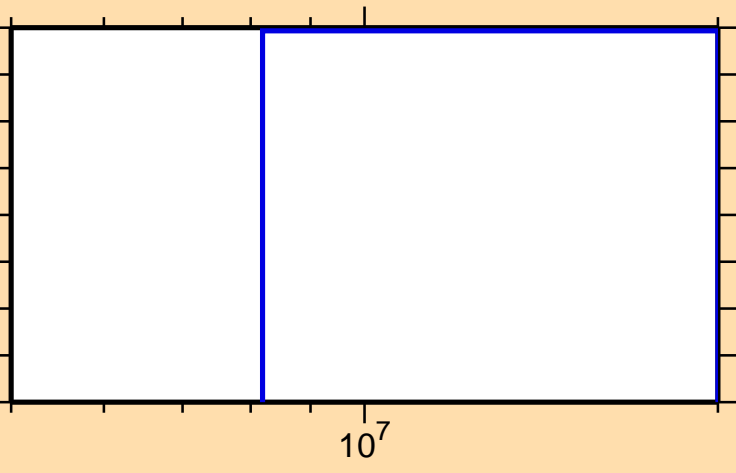
\sigma vs. E for ^{72}\text{Ge}(n,t)
