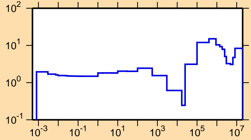
\Delta\sigma/\sigma vs. E for ^{72}\text{Ge}(n,\text{tot.})
