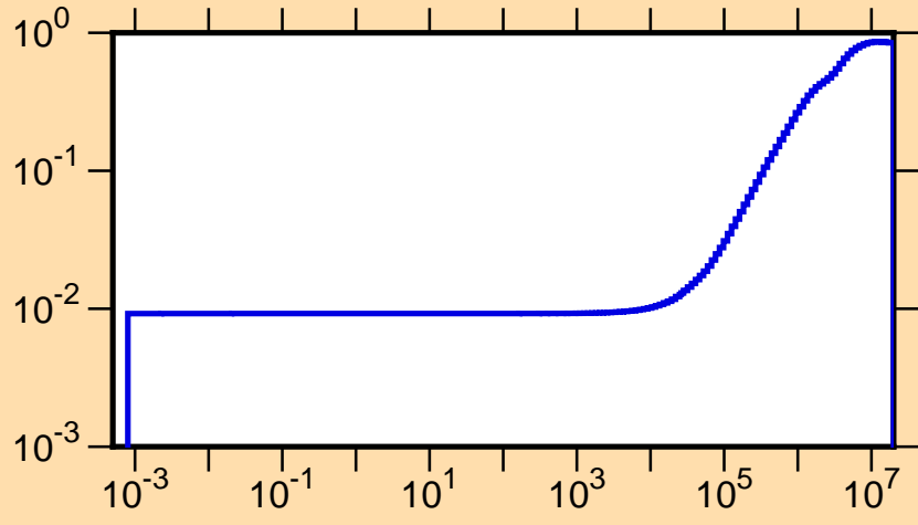
\mu vs. E for ^{73}\text{Ge}(\text{mt251})
