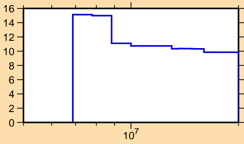
\Delta\sigma/\sigma vs. E for ^{73}\text{Ge}(n,2n)
