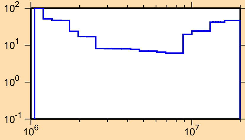
\Delta\sigma/\sigma vs. E for ^{73}\text{Ge}(n,ncont.)
