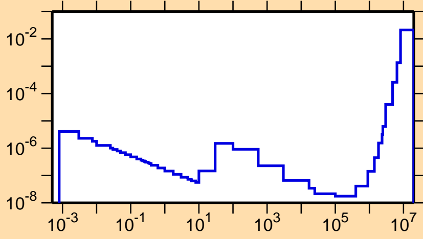
\sigma vs. E for ^{73}\text{Ge}(n,\alpha)
