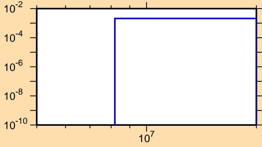
\sigma vs. E for ^{73}\text{Ge}(n,n\alpha)
