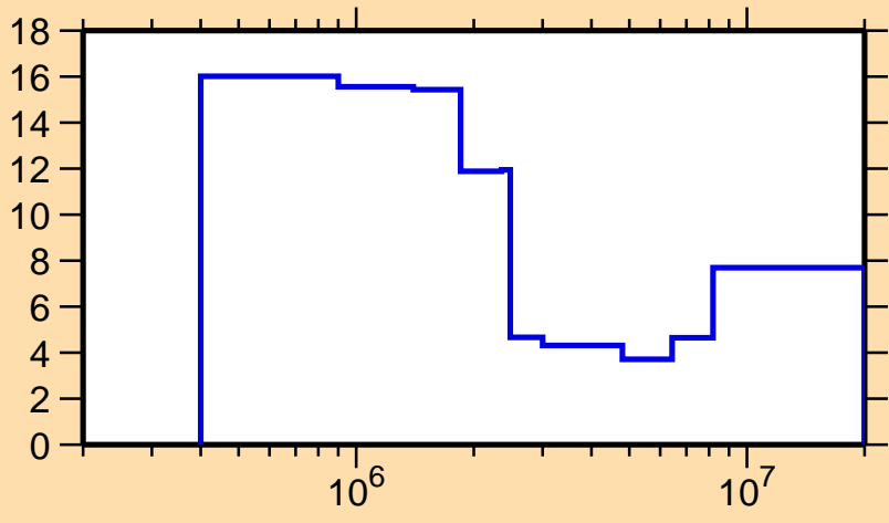
\Delta\sigma/\sigma vs. E for ^{73}\text{Ge}(n,\text{tot.})
