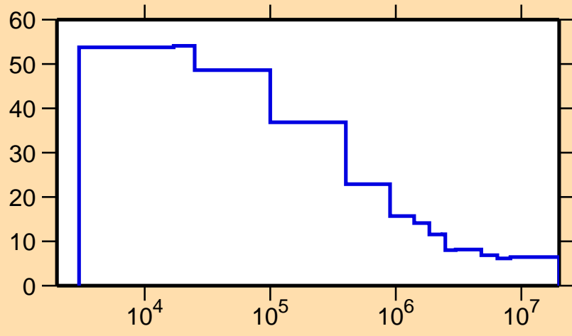
\Delta\sigma/\sigma vs. E for ^{73}\text{Ge}(n,\text{nonel.})
