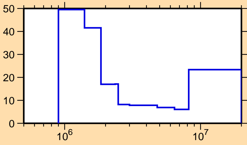
\Delta\sigma/\sigma vs. E for ^{73}\text{Ge}(n,n\text{cont.})
