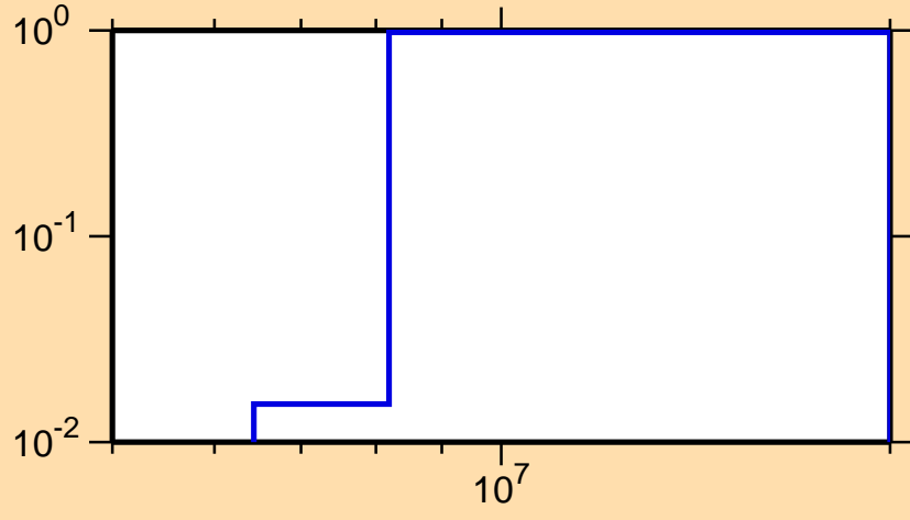
\sigma vs. E for ^{73}\text{Ge}(n,2n)
