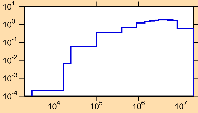
\sigma vs. E for ^{73}\text{Ge}(n,\text{inel.})
