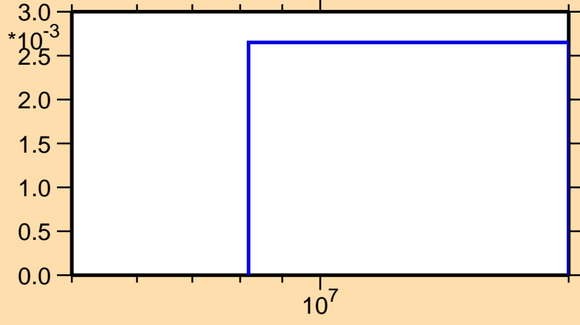
\sigma vs. E for ^{73}\text{Ge}(n,np)
