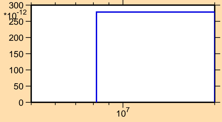
\sigma vs. E for ^{73}\text{Ge}(n,p\alpha)
