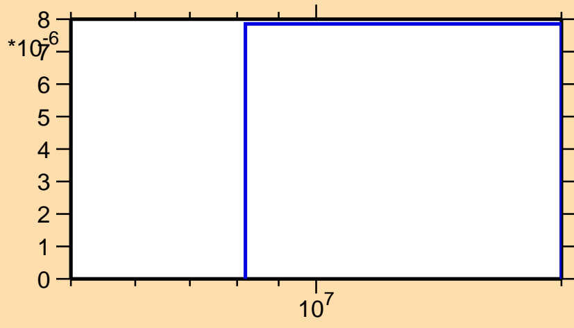
\sigma vs. E for ^{73}\text{Ge}(n,3n)
