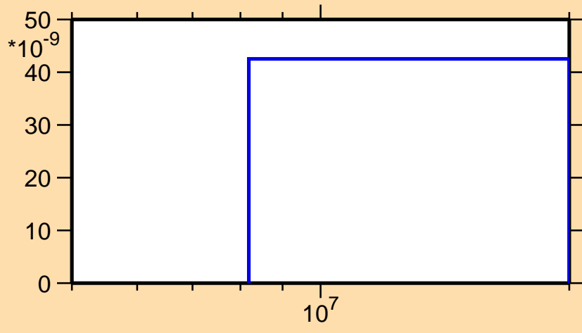
\sigma vs. E for ^{73}\text{Ge}(n,2n\alpha)
