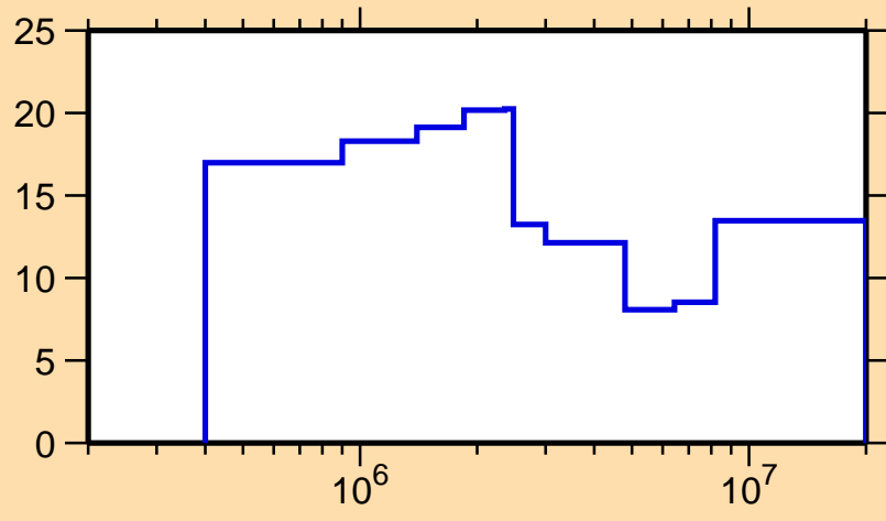
\Delta\sigma/\sigma vs. E for ^{73}\text{Ge}(n,\text{el.})
