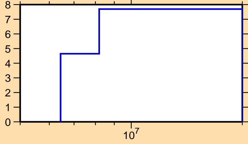
\Delta\sigma/\sigma vs. E for ^{73}\text{Ge}(n,\text{tot.})
