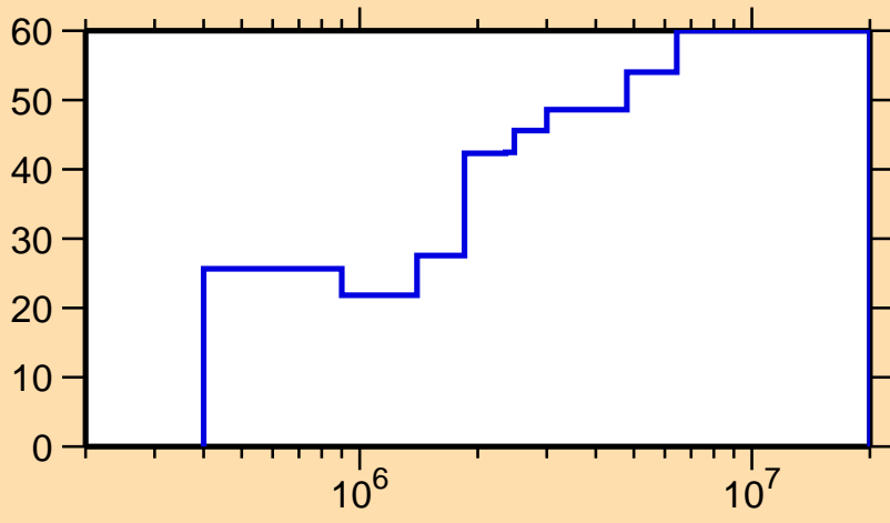
\Delta\sigma/\sigma vs. E for ^{73}\text{Ge}(n,n_1)
