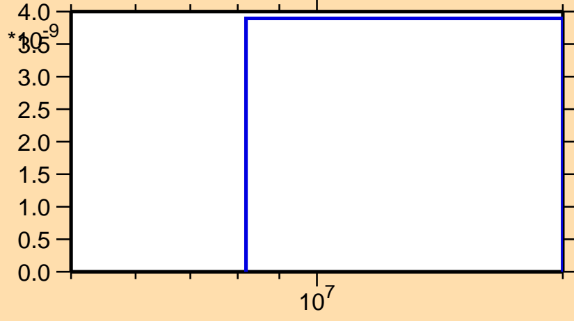
\sigma vs. E for ^{73}\text{Ge}(n,2np)
