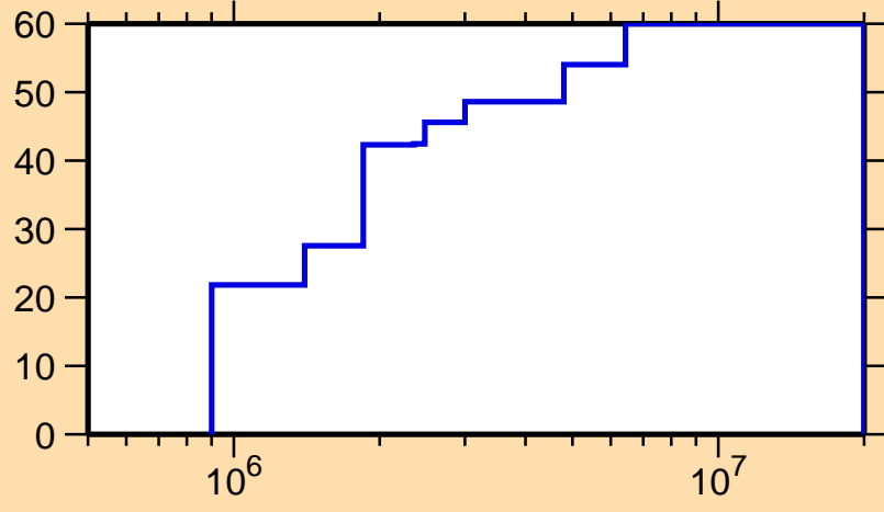
\Delta\sigma/\sigma vs. E for ^{73}\text{Ge}(n,n_1)
