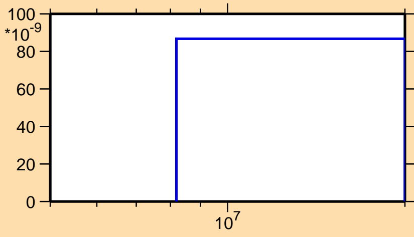
\sigma vs. E for ^{73}\text{Ge}(n,\text{nd})
