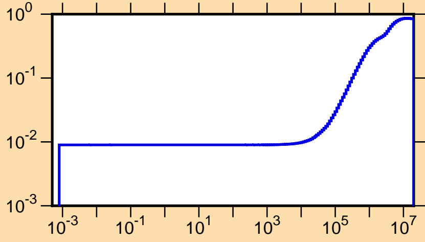
\mu vs. E for ^{75}\text{Ge}(\text{mt251})
