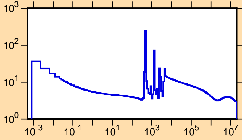
\sigma vs. E for ^{75}\text{Ge}(n,\text{tot.})
