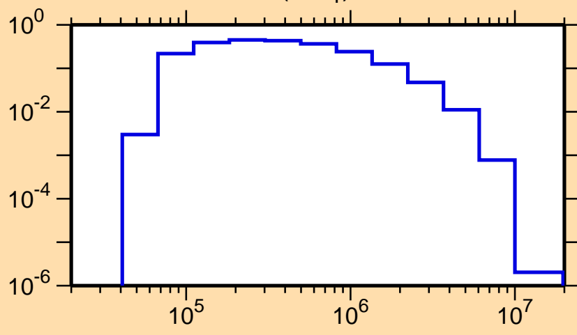
\sigma vs. E for ^{75}\text{Ge}(n,n_1)
