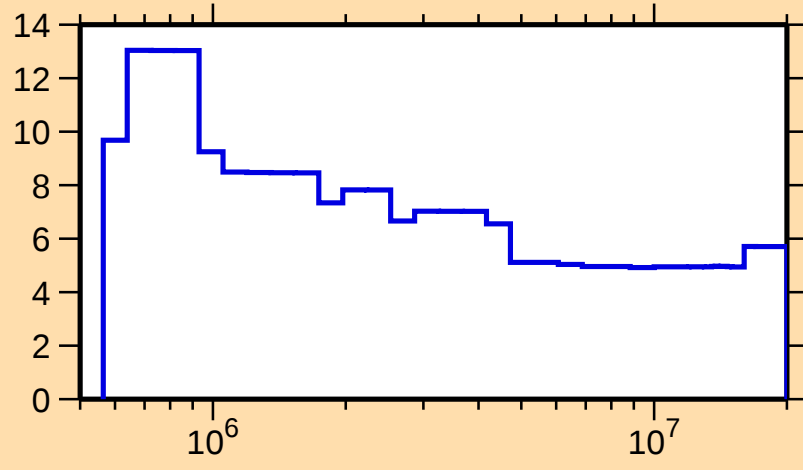
\Delta\sigma/\sigma vs. E for ^{76}\text{Ge}(\text{n,nonel.})
