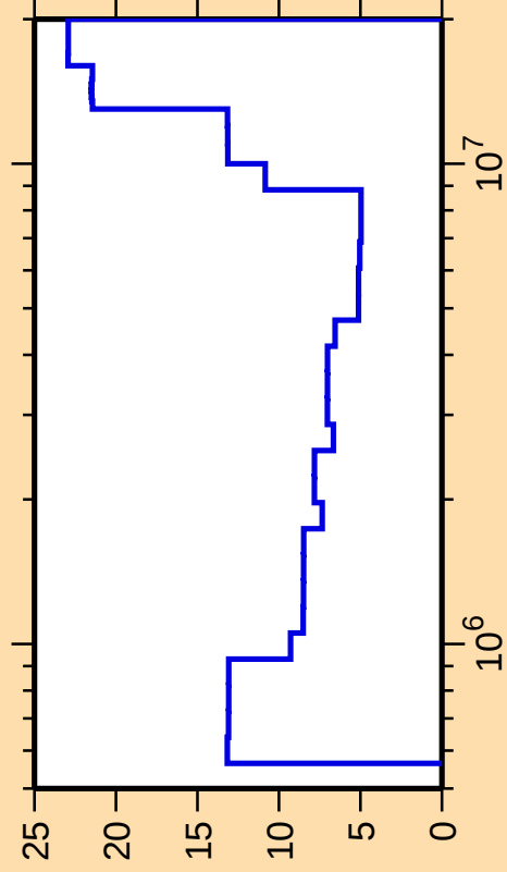
\Delta\sigma/\sigma vs. E for ^{76}\text{Ge}(\text{n,inel.})
