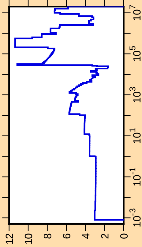
\Delta\sigma/\sigma vs. E for ^{76}\text{Ge}(n,\text{tot.})
