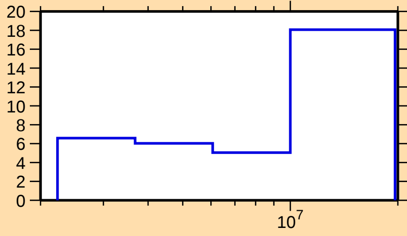
\Delta\sigma/\sigma vs. E for ^{76}\text{Ge}(\text{n},\text{inel.})
