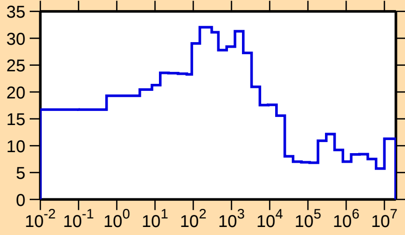
\Delta\sigma/\sigma vs. E for ^{76}\text{Ge}(\text{n,el.})
