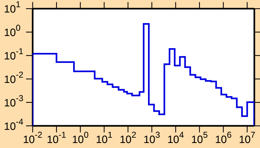
\sigma vs. E for ^{76}\text{Ge}(n,\gamma)
