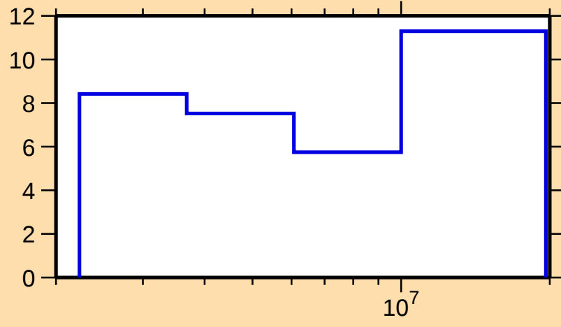
\Delta\sigma/\sigma vs. E for ^{76}\text{Ge}(\text{n},\text{el.})
