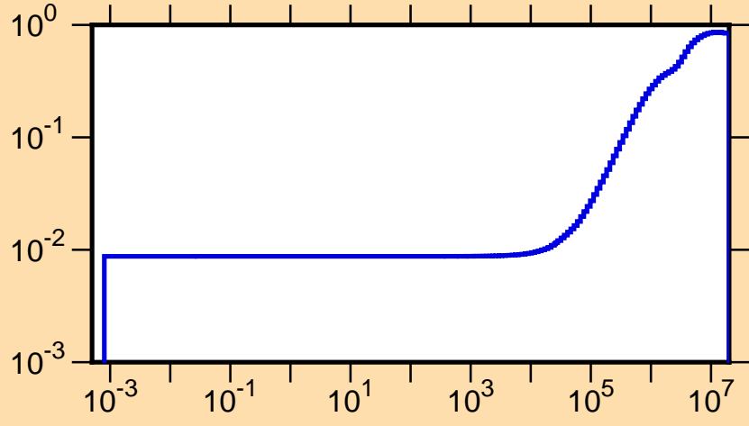
\mu vs. E for ^{77}\text{Ge}(\text{mt251})
