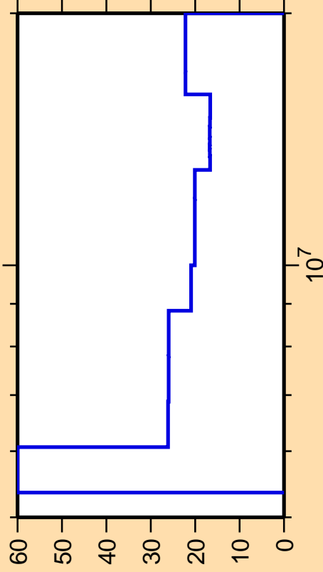
\Delta\sigma/\sigma vs. E for ^{79}\text{Ge}(n,2n)
