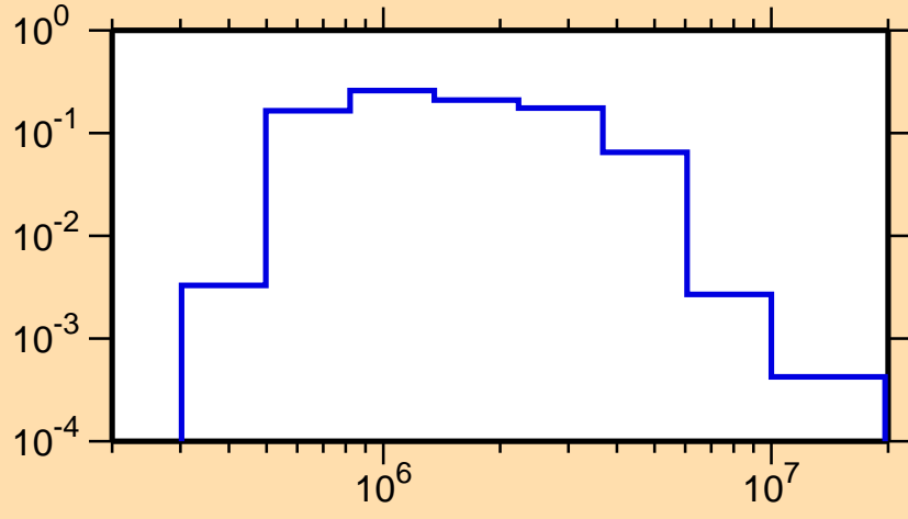
\sigma vs. E for ^{79}\text{Ge}(n,n_3)
