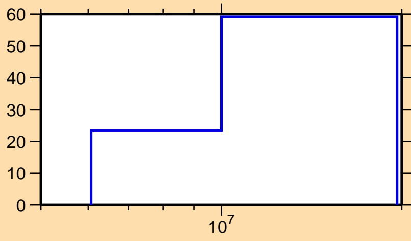
\Delta\sigma/\sigma vs. E for ^{79}\text{Ge}(n,ncont.)
