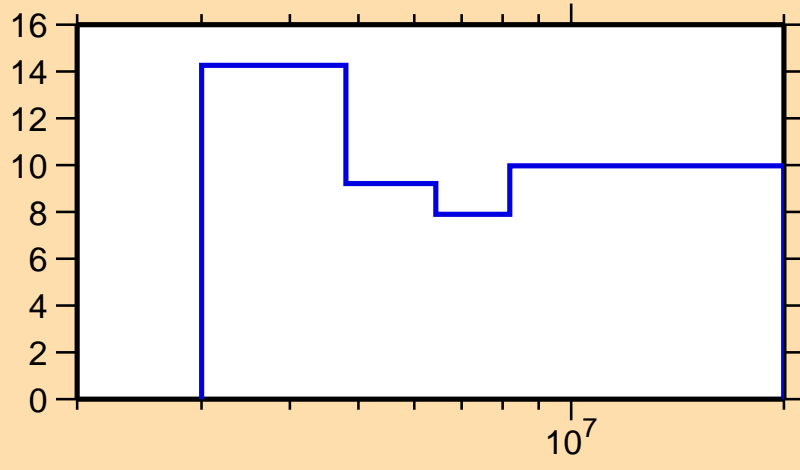
\Delta\sigma/\sigma vs. E for ^{79}\text{Ge}(n,n\text{onel.})
