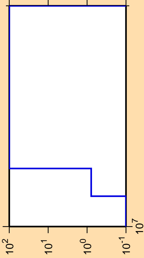
\Delta\sigma/\sigma vs. E for ^{79}\text{Ge}(n,t)
