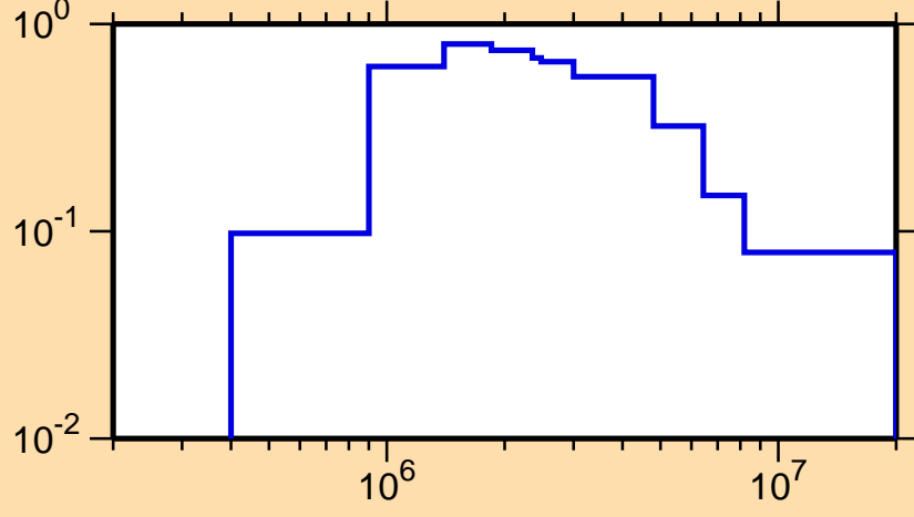
\sigma vs. E for ^{80}\text{Ge}(n,n_1)
