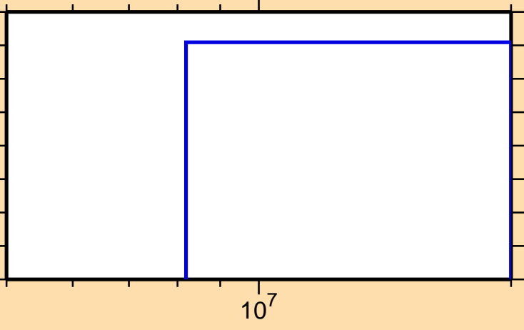
\sigma vs. E for ^{80}\text{Ge}(n,3n)
