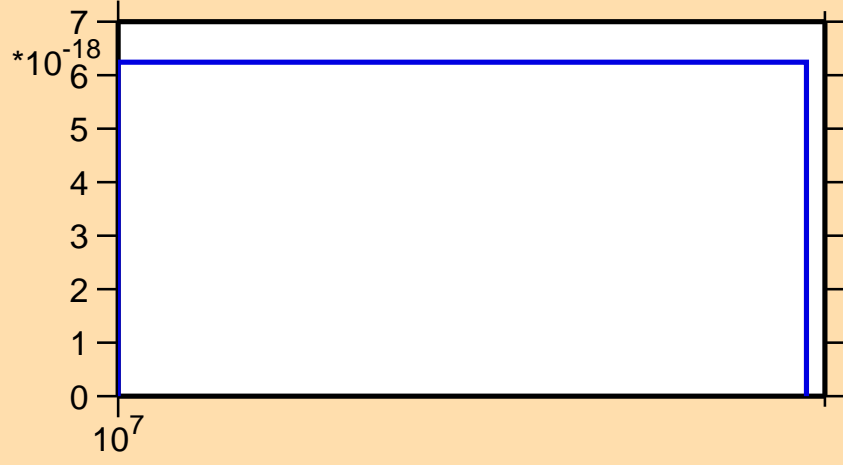
\sigma vs. E for ^{82}\text{Ge}(n,\text{nd})
