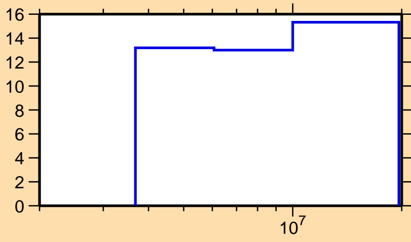
\Delta\sigma/\sigma vs. E for ^{82}\text{Ge}(n,n\text{onel.})
