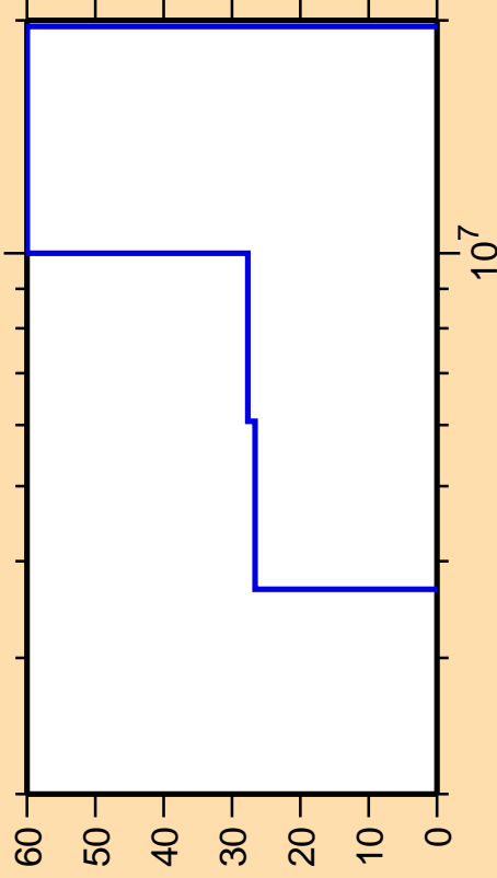
\Delta\sigma/\sigma vs. E for ^{82}\text{Ge}(n,n\text{cont.})
