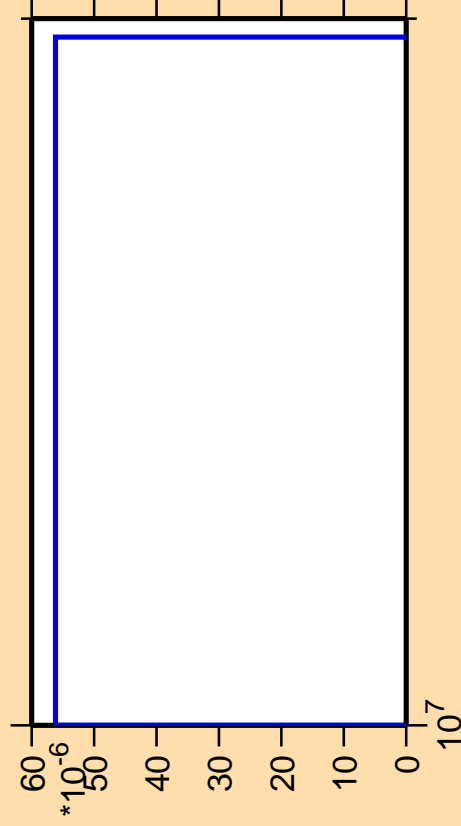
\Delta\sigma/\sigma vs. E for ^{82}\text{Ge}(n,\text{nd})
