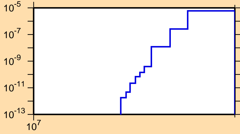
\sigma vs. E for ^{83}\text{Ge}(n,n\alpha)
