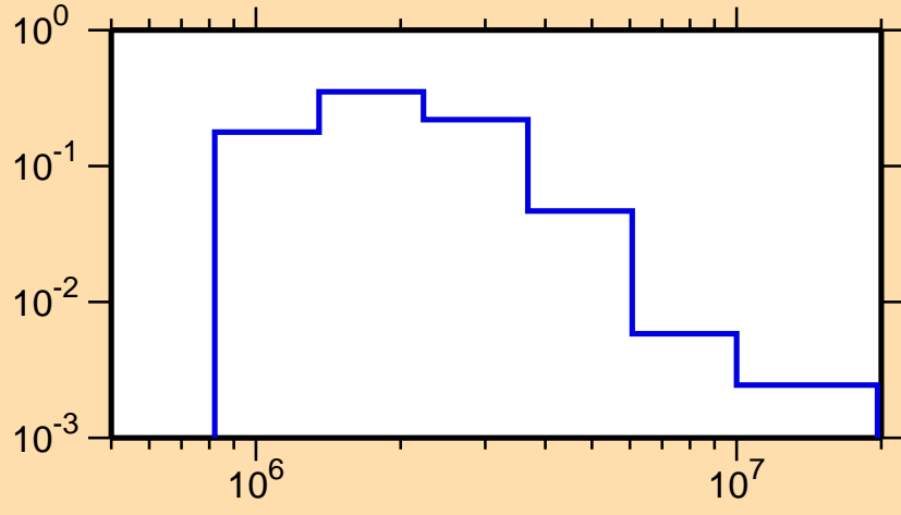
\sigma vs. E for ^{83}\text{Ge}(n,n_2)
