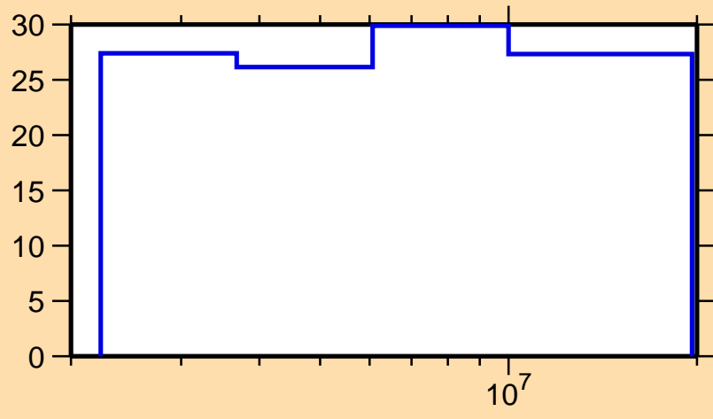
\Delta\sigma/\sigma vs. E for ^{83}\text{Ge}(n,n\text{cont.})
