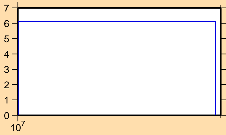
\Delta\sigma/\sigma vs. E for ^{83}\text{Ge}(n,\text{nonel.})
