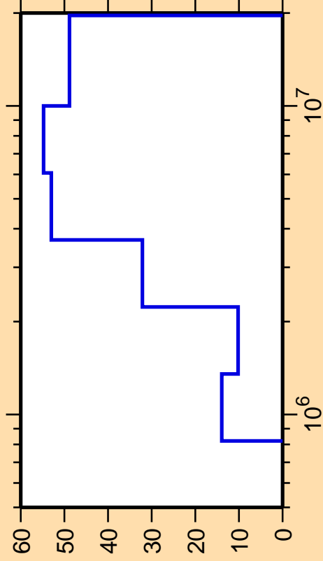
\Delta\sigma/\sigma vs. E for ^{83}\text{Ge}(n,n_2)
