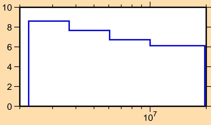
\Delta\sigma/\sigma vs. E for ^{83}\text{Ge}(n,n\text{onel.})
