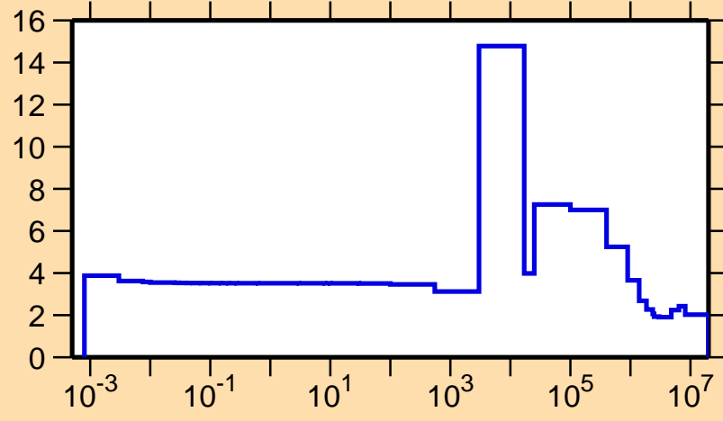
\sigma vs. E for ^{83}\text{Ge}(n,\text{el.})
