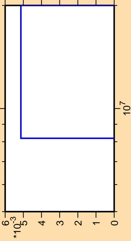
\Delta\sigma/\sigma vs. E for ^{83}\text{Ge}(n,2np)
