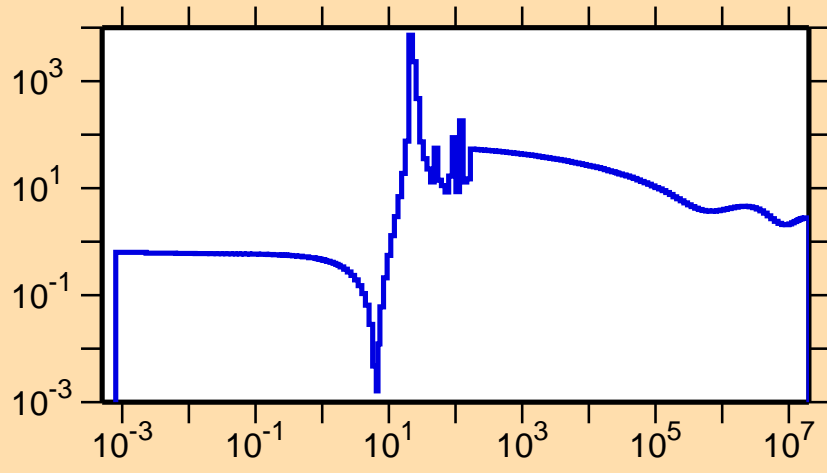
\sigma vs. E for ^{154}\text{Hf}(n,\text{el.})
