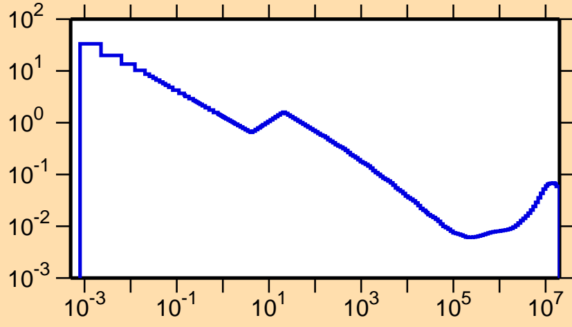
\sigma vs. E for ^{154}\text{Hf}(n,\alpha)
