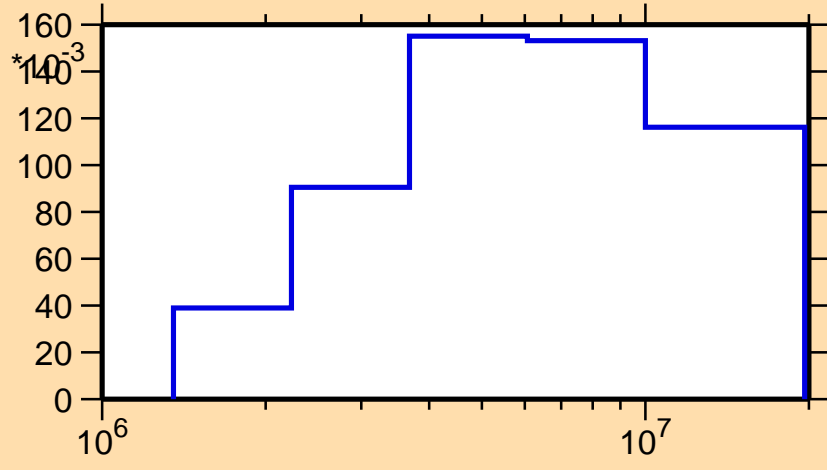
\sigma vs. E for ^{154}\text{Hf}(n,\text{inel.})
