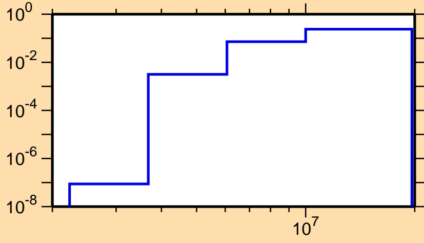
\sigma vs. E for ^{154}\text{Hf}(n,np)
