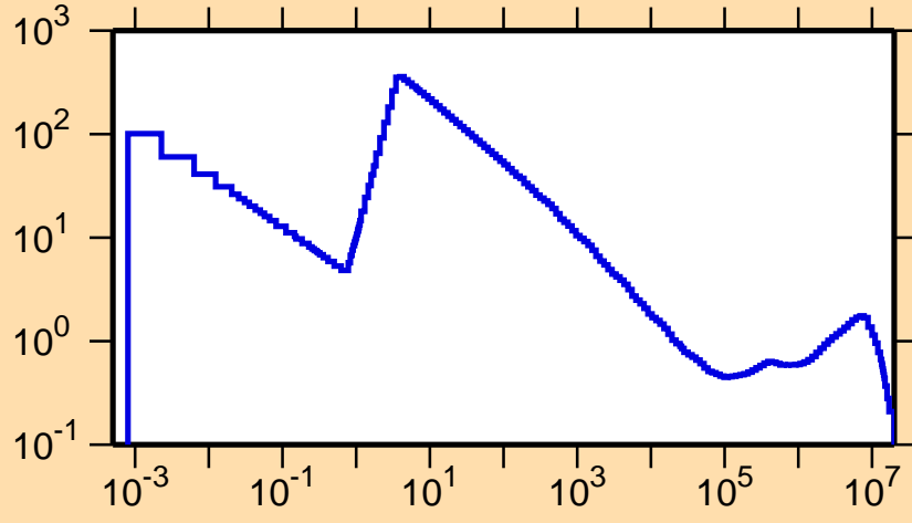
\sigma vs. E for ^{158}\text{Hf}(n,p)
