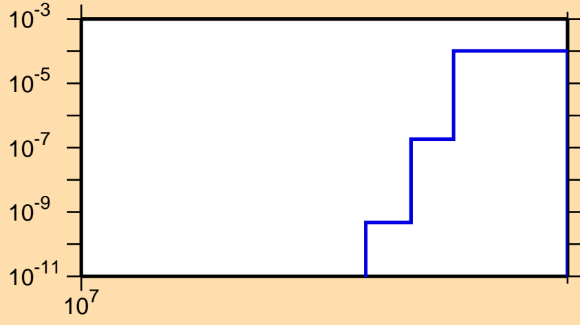
\sigma vs. E for ^{158}\text{Hf}(n,2np)
