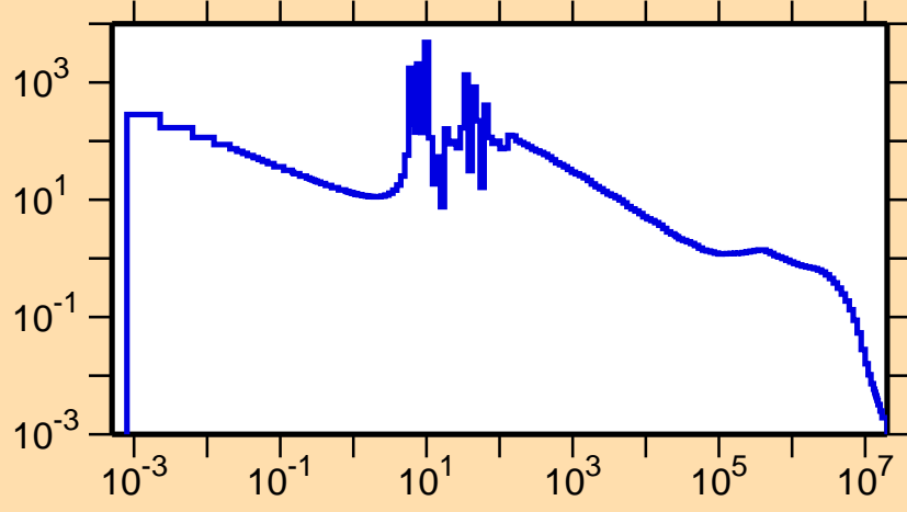
\sigma vs. E for ^{158}\text{Hf}(n,\gamma)
