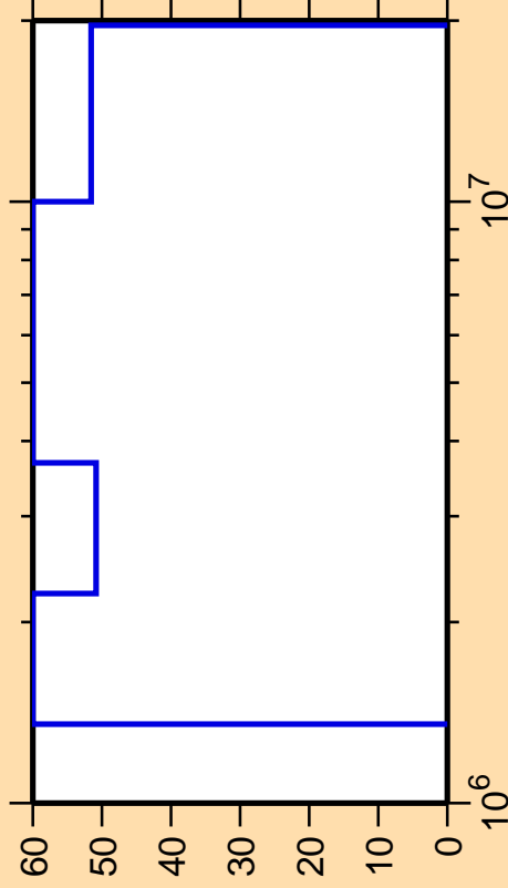
\Delta\sigma/\sigma vs. E for ^{158}\text{Hf}(n,n_3)
