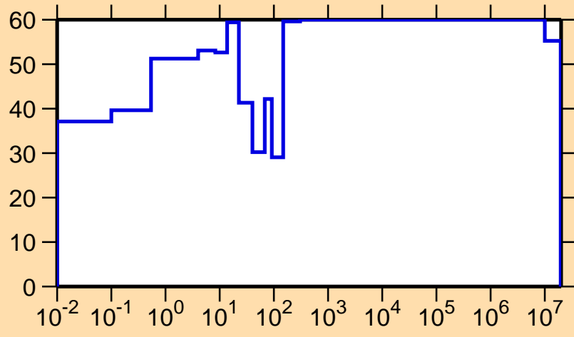
\Delta\sigma/\sigma vs. E for ^{158}\text{Hf}(n,\gamma)
