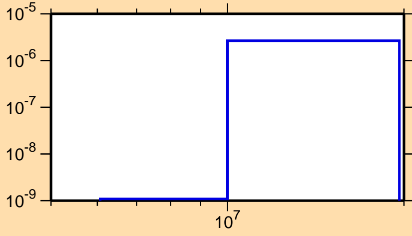
\sigma vs. E for ^{158}\text{Hf}(\text{mt117})
