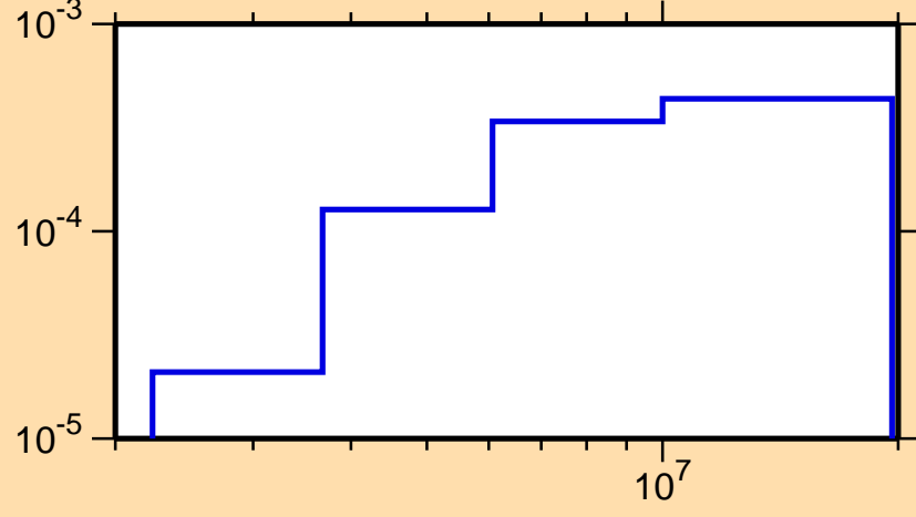
\sigma vs. E for ^{158}\text{Hf}(n,n_4)
