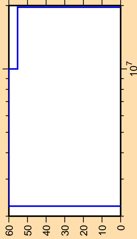
\Delta\sigma/\sigma vs. E for ^{158}\text{Hf}(n,n_4)
