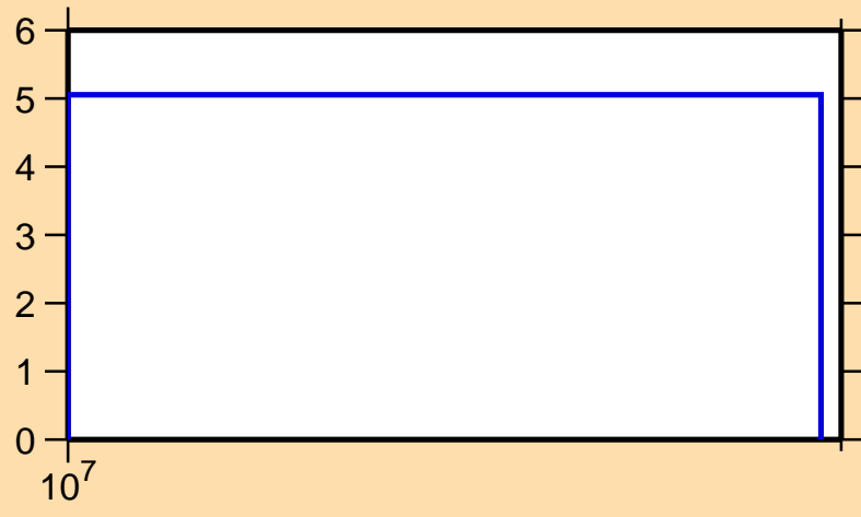
\Delta\sigma/\sigma vs. E for ^{158}\text{Hf}(n,\text{nonel.})
