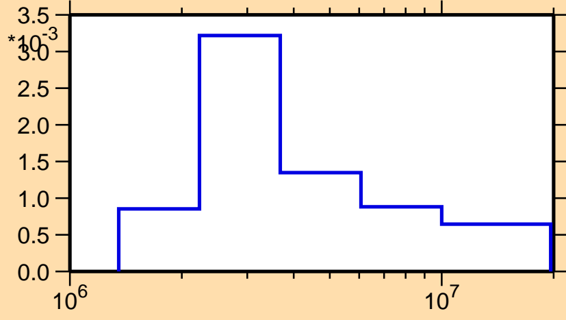
\sigma vs. E for ^{158}\text{Hf}(n,n_3)
