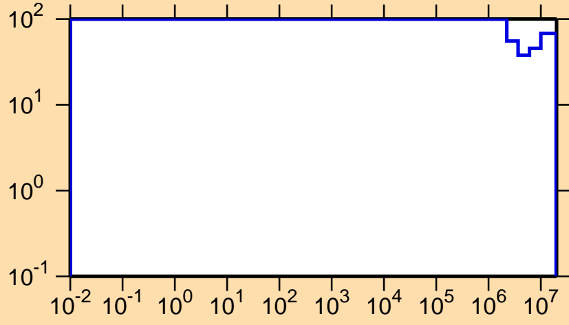
\Delta\sigma/\sigma vs. E for ^{158}\text{Hf}(n,p)
