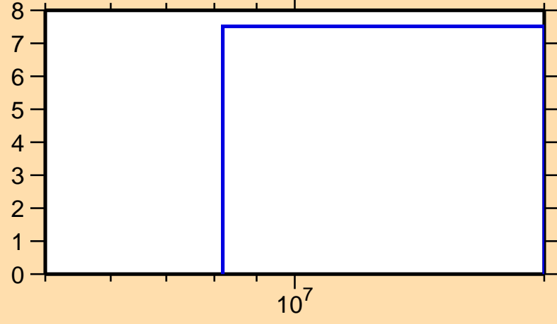
\Delta\sigma/\sigma vs. E for ^{158}\text{Hf}(n,\text{el.})
