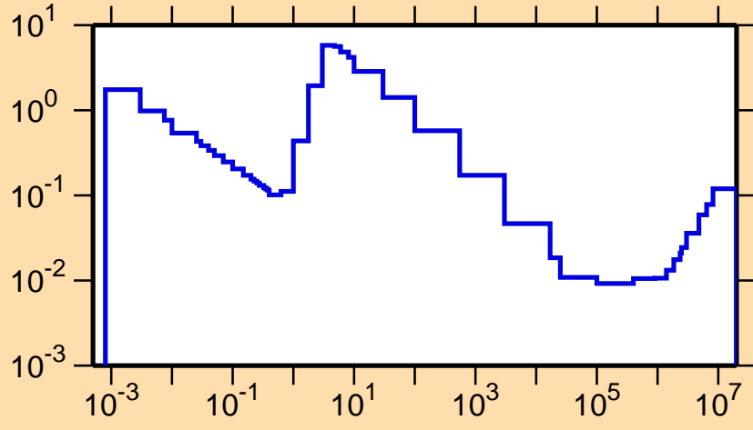
\sigma vs. E for ^{158}\text{Hf}(n,\alpha)
