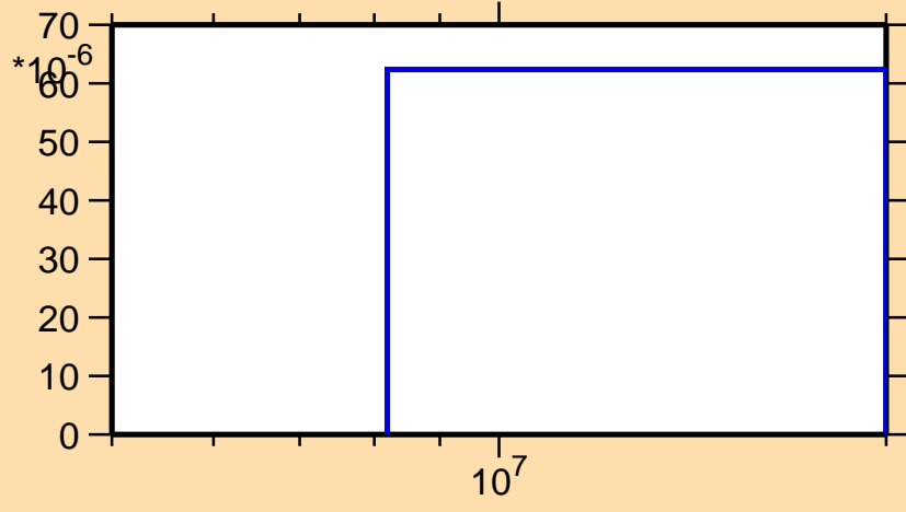
\sigma vs. E for ^{158}\text{Hf}(n,t)
