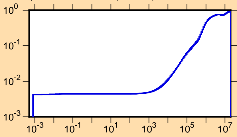
\mu vs. E for ^{159}\text{Hf}(\text{mt251})
