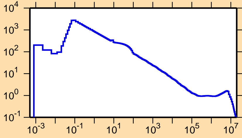
\sigma vs. E for ^{159}\text{Hf}(n,p)
