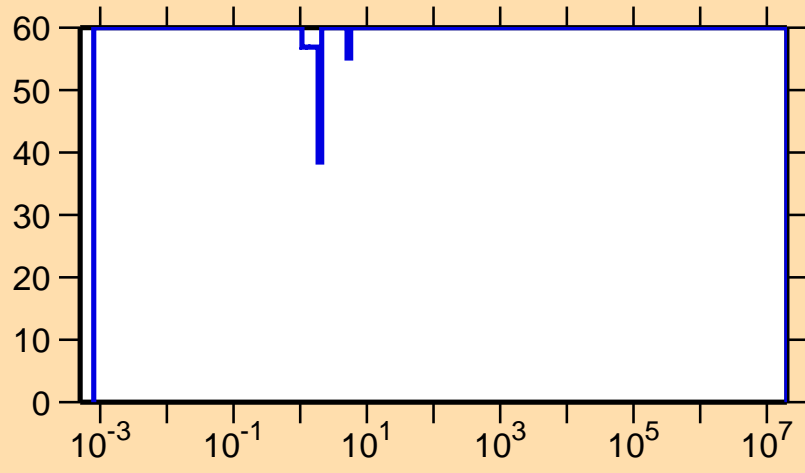
\Delta\sigma/\sigma vs. E for ^{159}\text{Hf}(n,\gamma)
