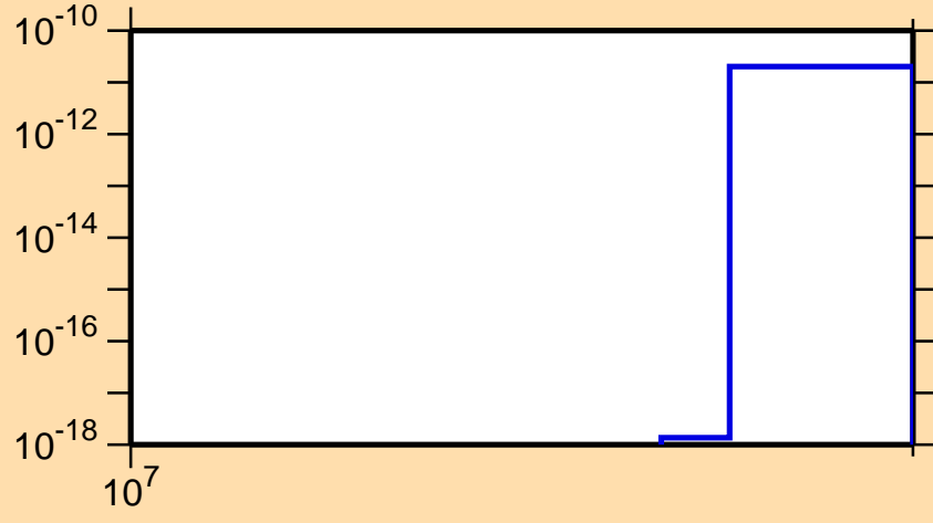
\sigma vs. E for ^{159}\text{Hf}(n,nt)
