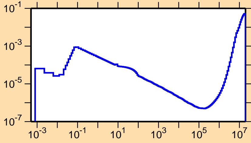
\sigma vs. E for ^{159}\text{Hf}(n,p\alpha)
