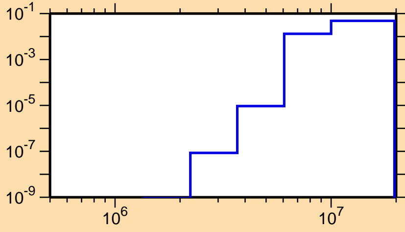
\sigma vs. E for ^{159}\text{Hf}(n,n\alpha)
