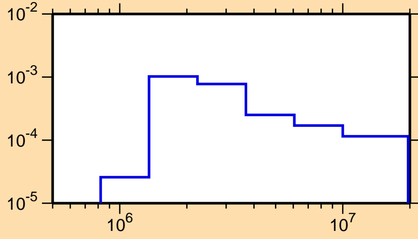
\sigma vs. E for ^{159}\text{Hf}(n,n_3)
