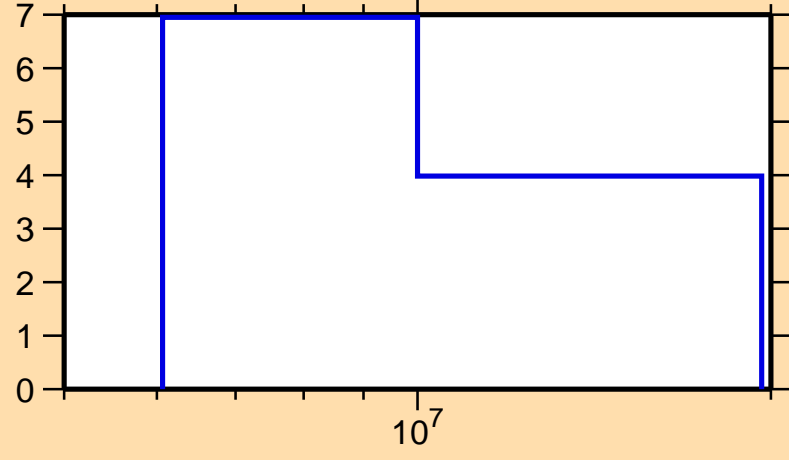
\Delta\sigma/\sigma vs. E for ^{159}\text{Hf}(n,\text{nonel.})
