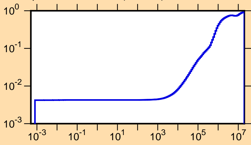
\mu vs. E for ^{160}\text{Hf}(\text{mt251})
