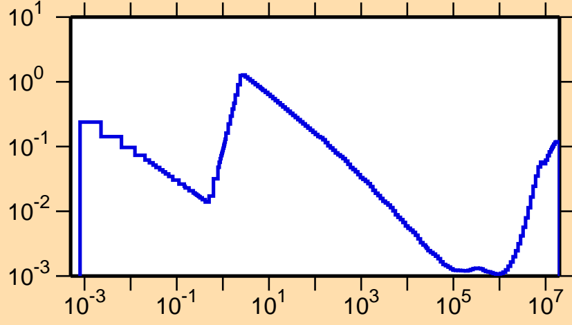
\sigma vs. E for ^{160}\text{Hf}(n,\alpha)
