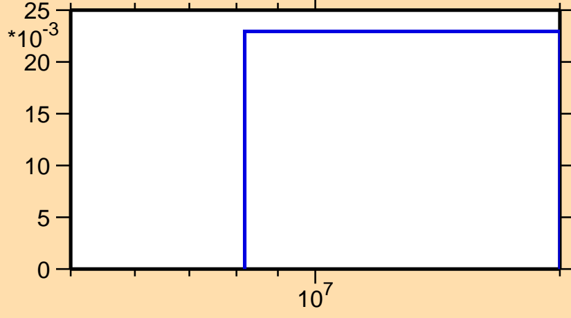
\sigma vs. E for ^{160}\text{Hf}(n,2n)
