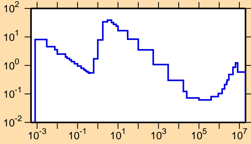
\sigma vs. E for ^{160}\text{Hf}(n,p)
