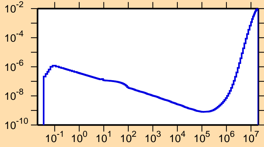
\sigma vs. E for ^{161}\text{Hf}(n,p\alpha)
