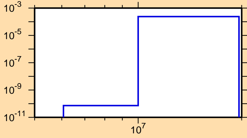
\sigma vs. E for ^{161}\text{Hf}(n,t)
