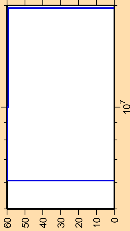
\Delta\sigma/\sigma vs. E for ^{161}\text{Hf}(n,n_1)
