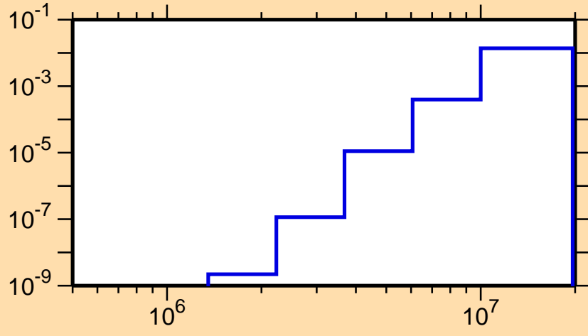
\sigma vs. E for ^{161}\text{Hf}(n,n\alpha)
