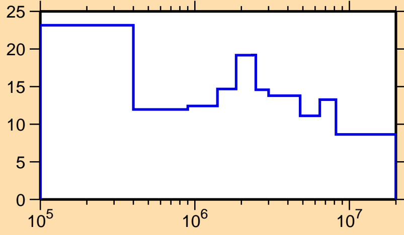
\Delta\sigma/\sigma vs. E for ^{161}\text{Hf}(n,\text{tot.})
