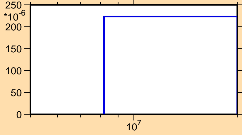
\sigma vs. E for ^{161}\text{Hf}(n,2n\alpha)
