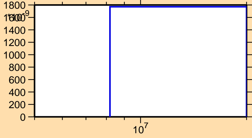
\sigma vs. E for ^{161}\text{Hf} (mt 45)
