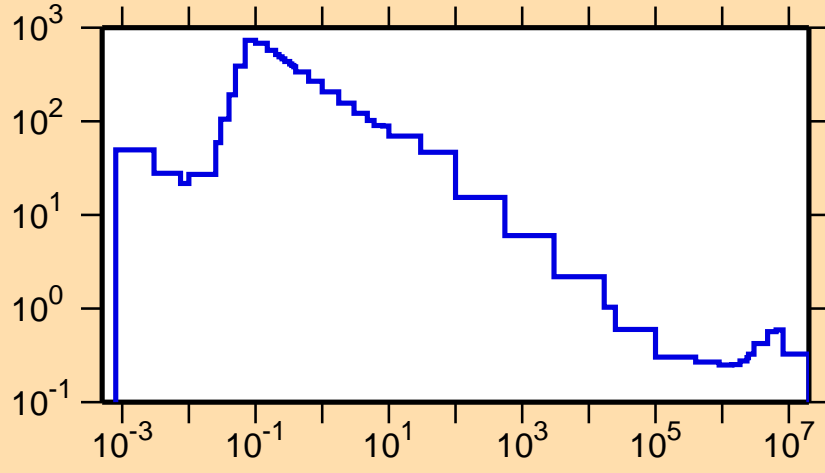
\sigma vs. E for ^{161}\text{Hf}(n,p)
