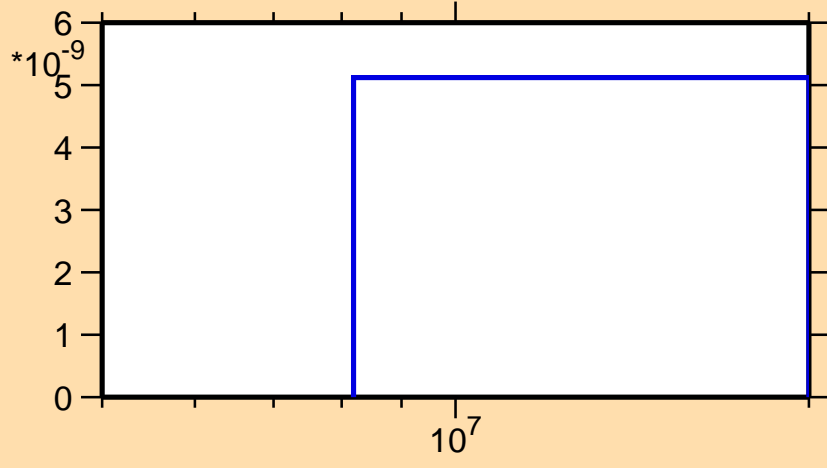
\sigma vs. E for ^{161}\text{Hf}(\text{mt117})
