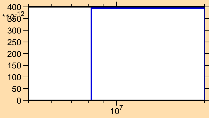
\sigma vs. E for ^{161}\text{Hf} (mt 34)
