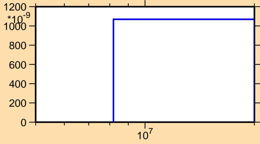
\sigma vs. E for ^{161}\text{Hf}(n,\text{pd})
