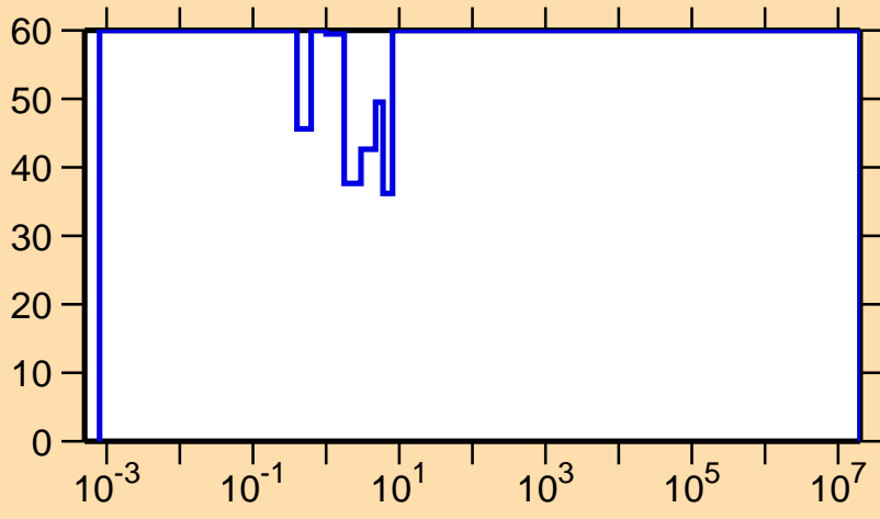
\Delta\sigma/\sigma vs. E for ^{161}\text{Hf}(n,\gamma)
