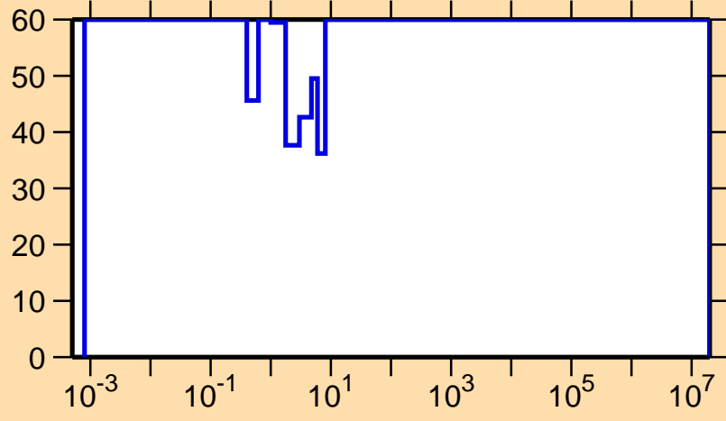
\Delta\sigma/\sigma vs. E for ^{161}\text{Hf}(n,\gamma)
