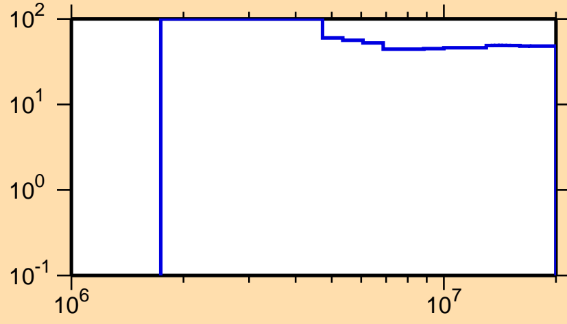
\Delta\sigma/\sigma vs. E for ^{162}\text{Hf}(n,n\text{cont.})
