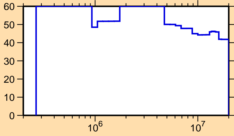
\Delta\sigma/\sigma vs. E for ^{162}\text{Hf}(n,n_1)
