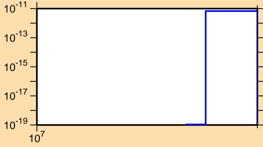
\sigma vs. E for ^{162}\text{Hf}(n,nt)
