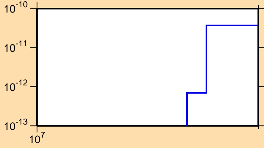
\sigma vs. E for ^{162}\text{Hf} (mt 34)
